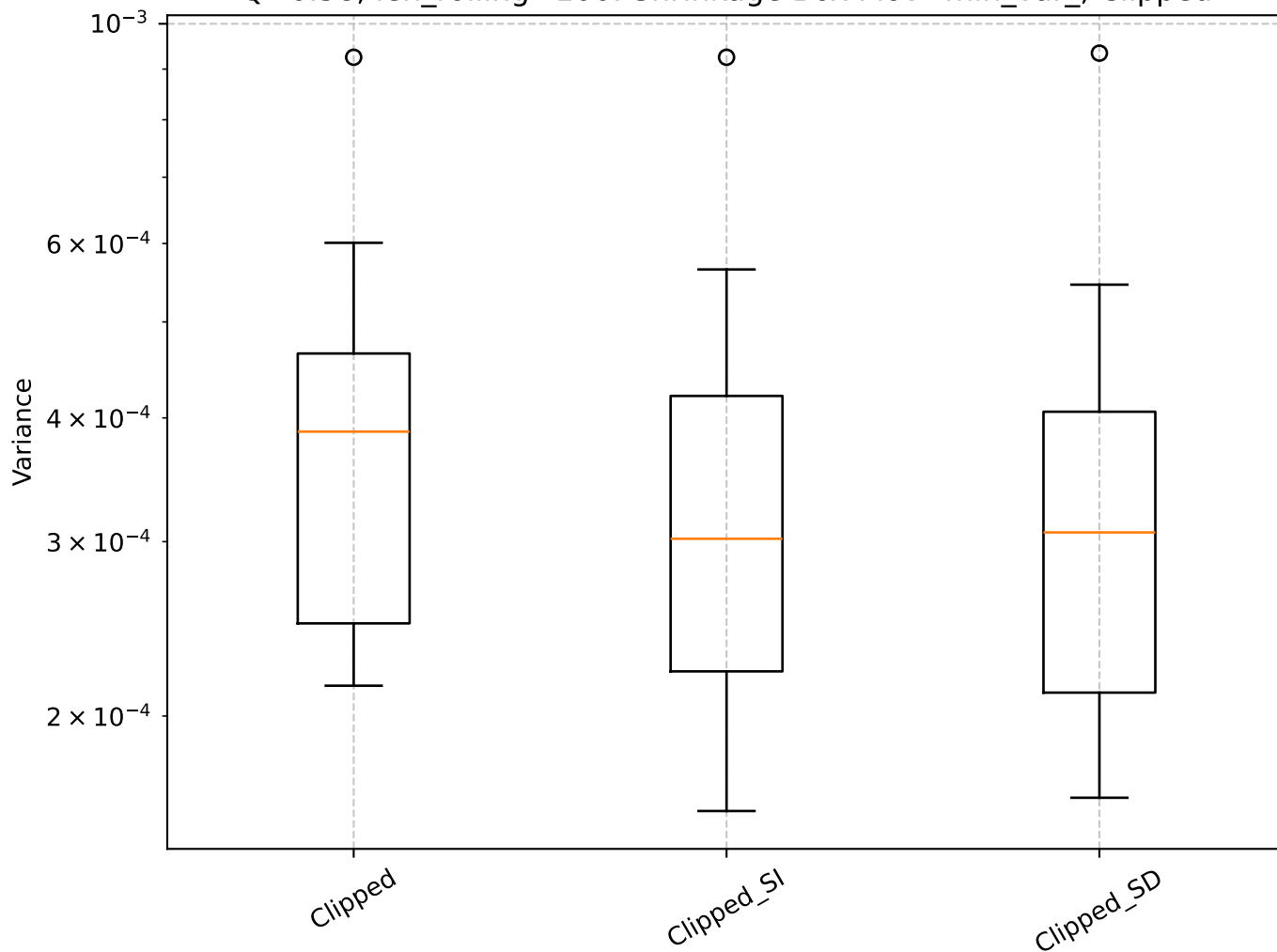
Q=0.58, len_rolling=100: Shrinkage Box Plot - min_var_, Clipped
