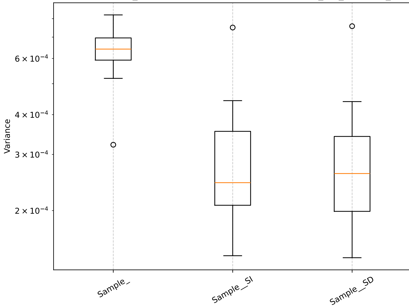
Q=0.58, len_rolling=100: Shrinkage Box Plot - min_var_, Sample_
