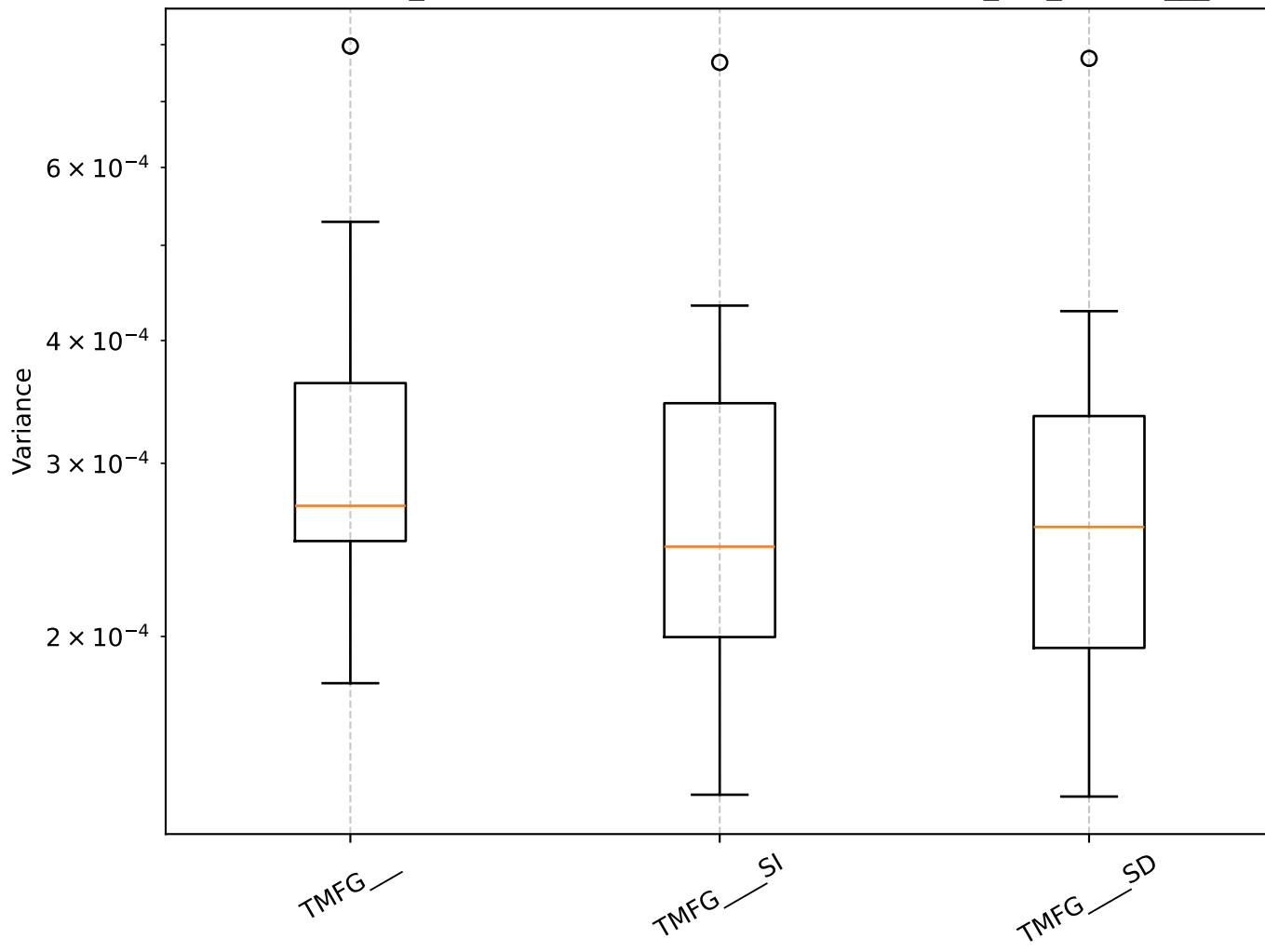
Q=0.63, len_rolling=100: Shrinkage Box Plot - min_var_, TMFG__
