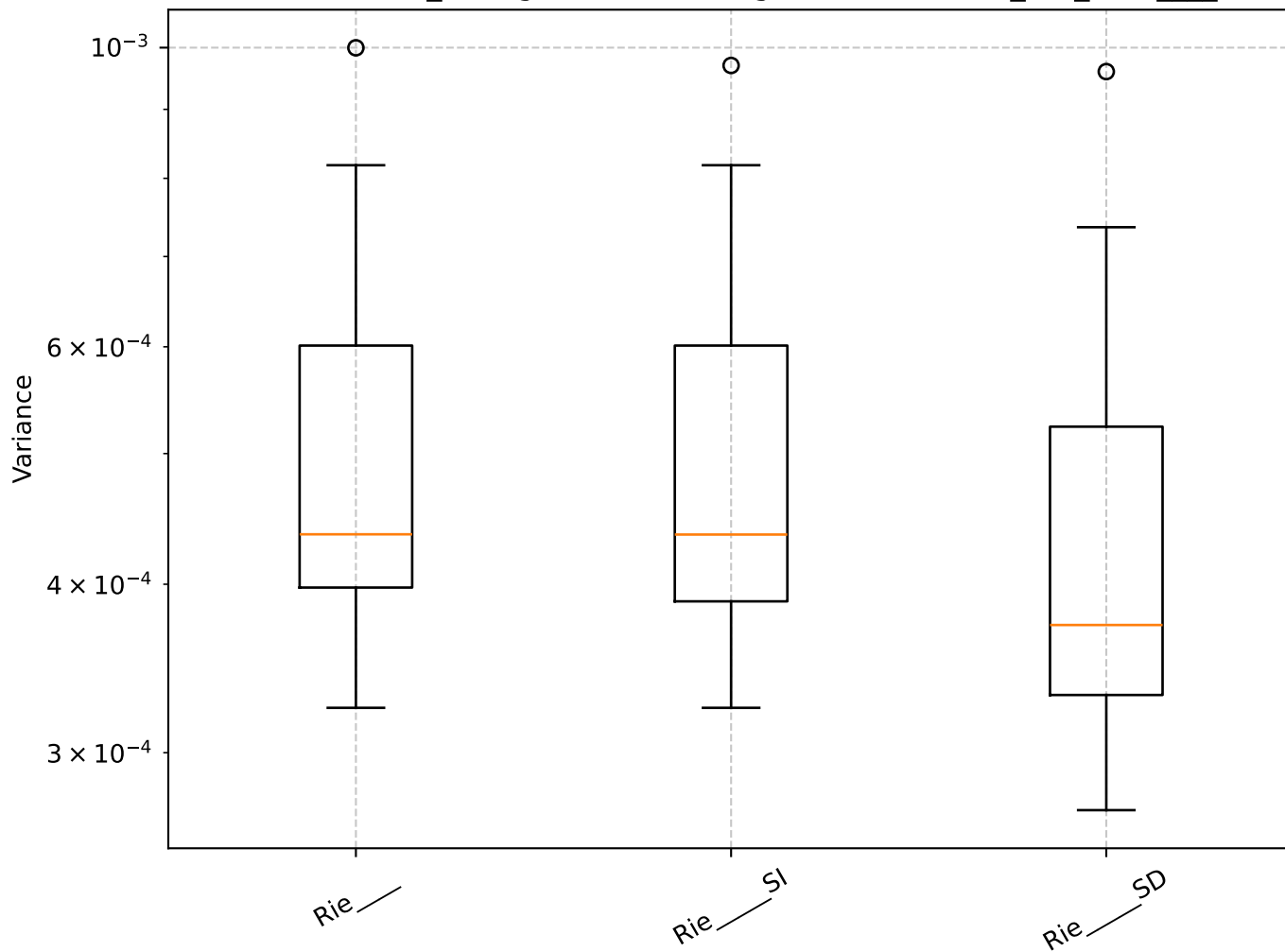
Q=0.66, len_rolling=100: Shrinkage Box Plot - min_var_, Rie__
