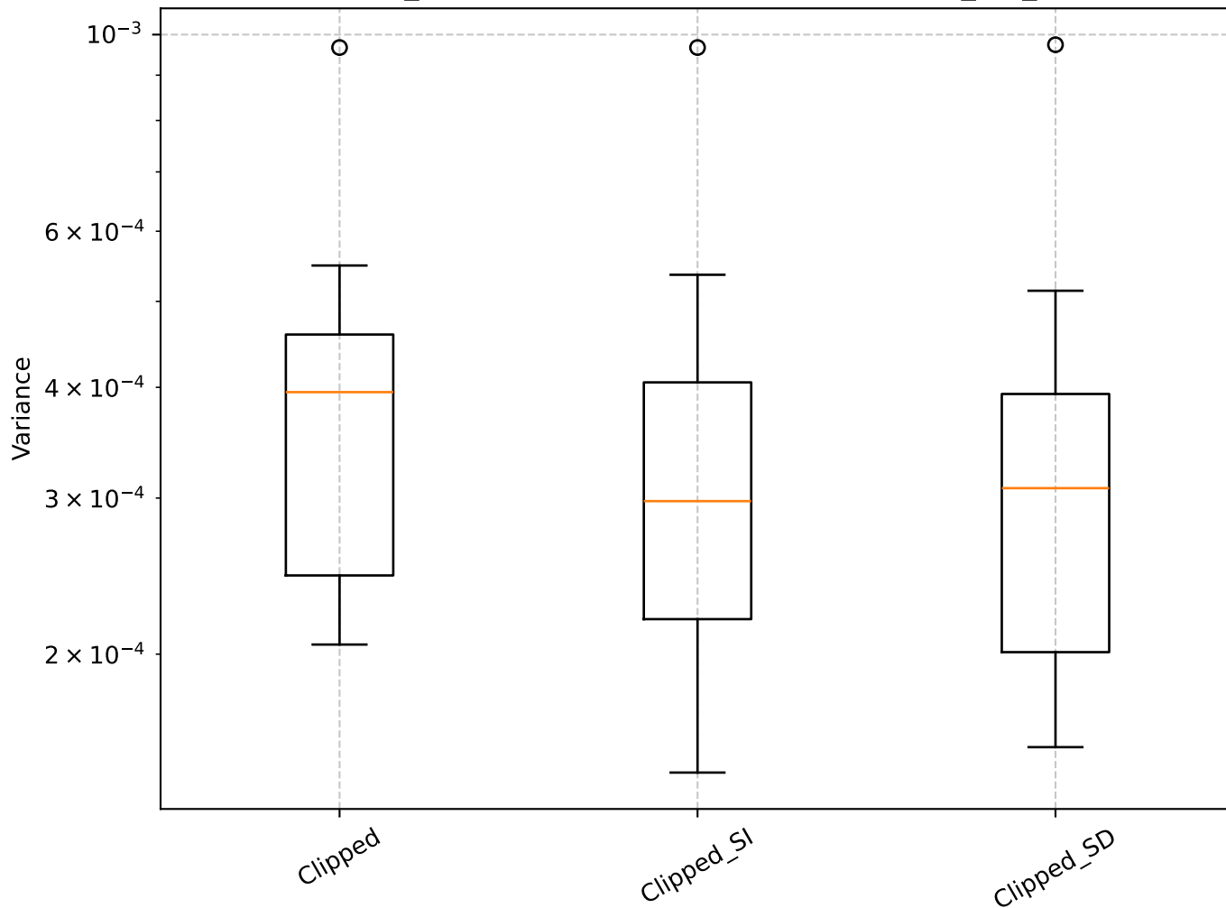
Q=0.67, len_rolling=100: Shrinkage Box Plot - min_var_, Clipped
