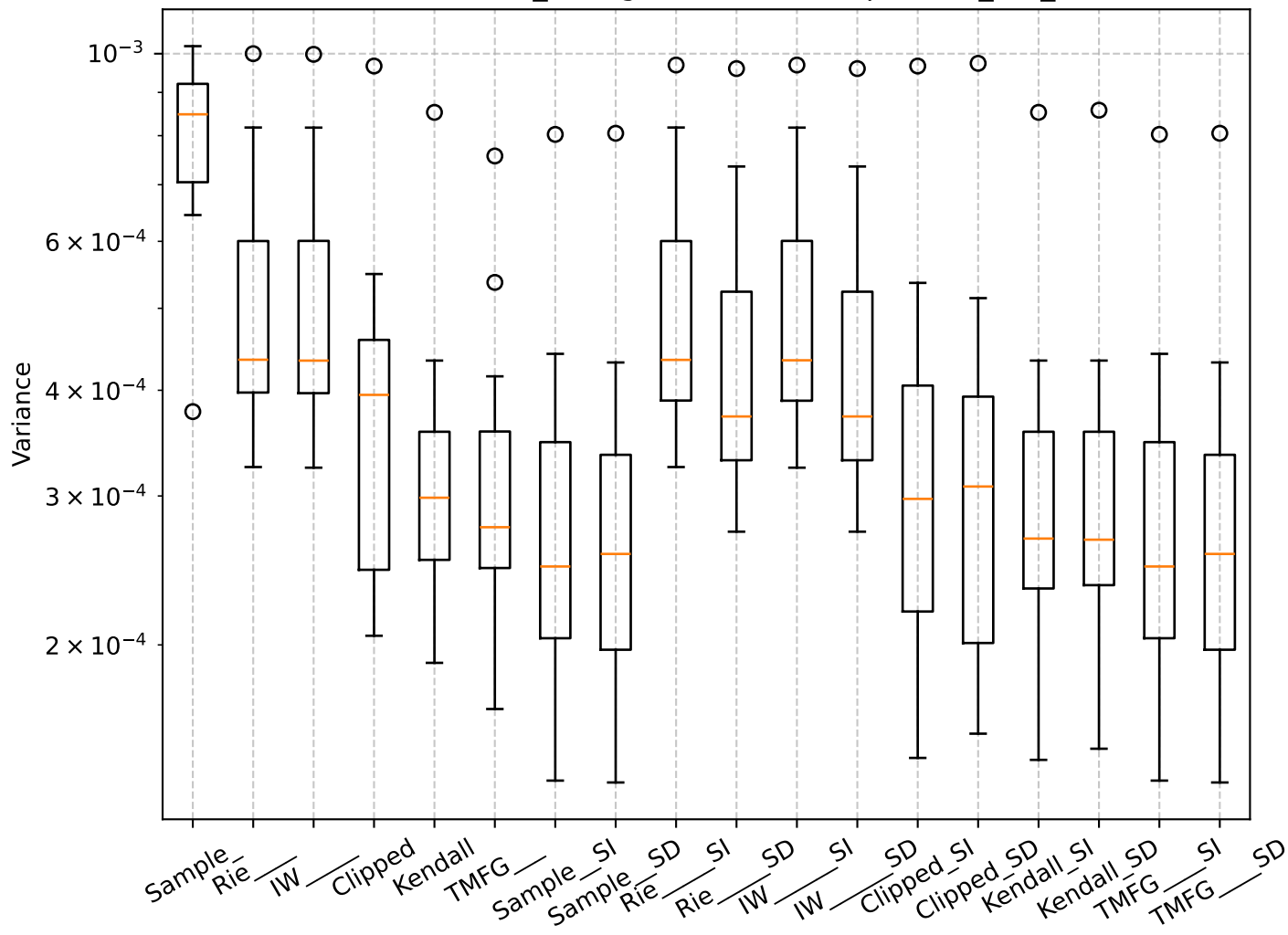
Q=0.67, len_rolling=100: Box Plot per min_var_
