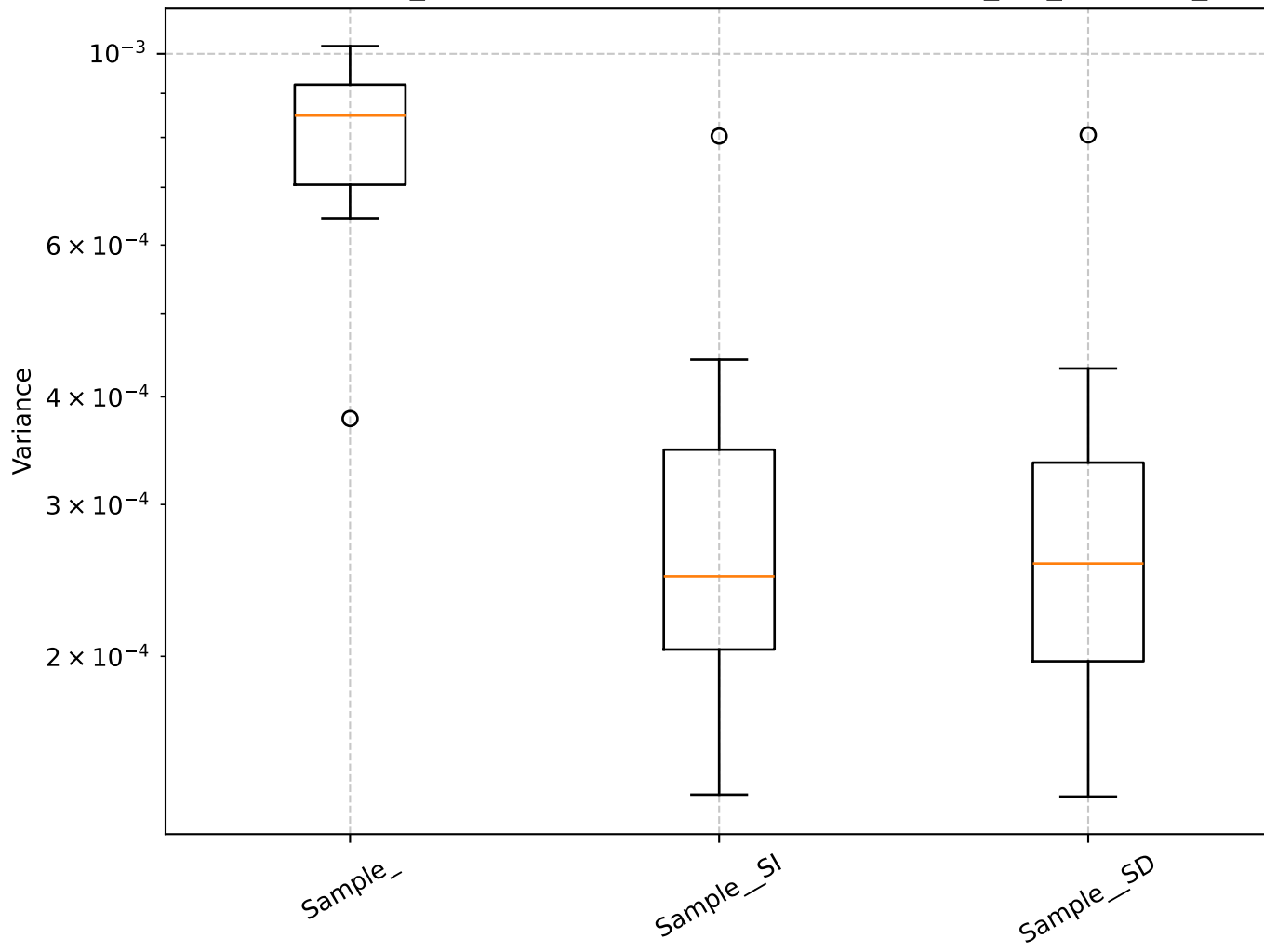
Q=0.67, len_rolling=100: Shrinkage Box Plot - min_var_, Sample_
