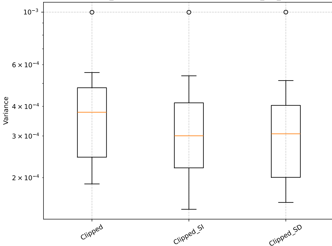
Q=0.70, len_rolling=100: Shrinkage Box Plot - min_var_, Clipped
