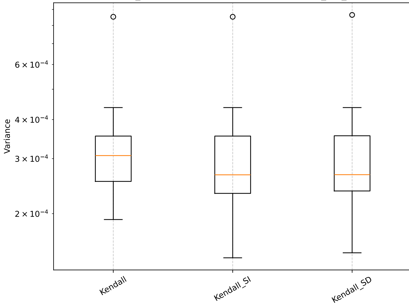
Q=0.70, len_rolling=100: Shrinkage Box Plot - min_var_, Kendall
