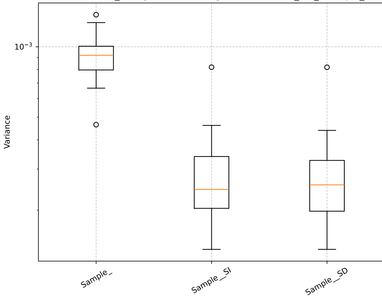
Q=0.71, len_rolling=100: Shrinkage Box Plot - min_var_, Sample_
