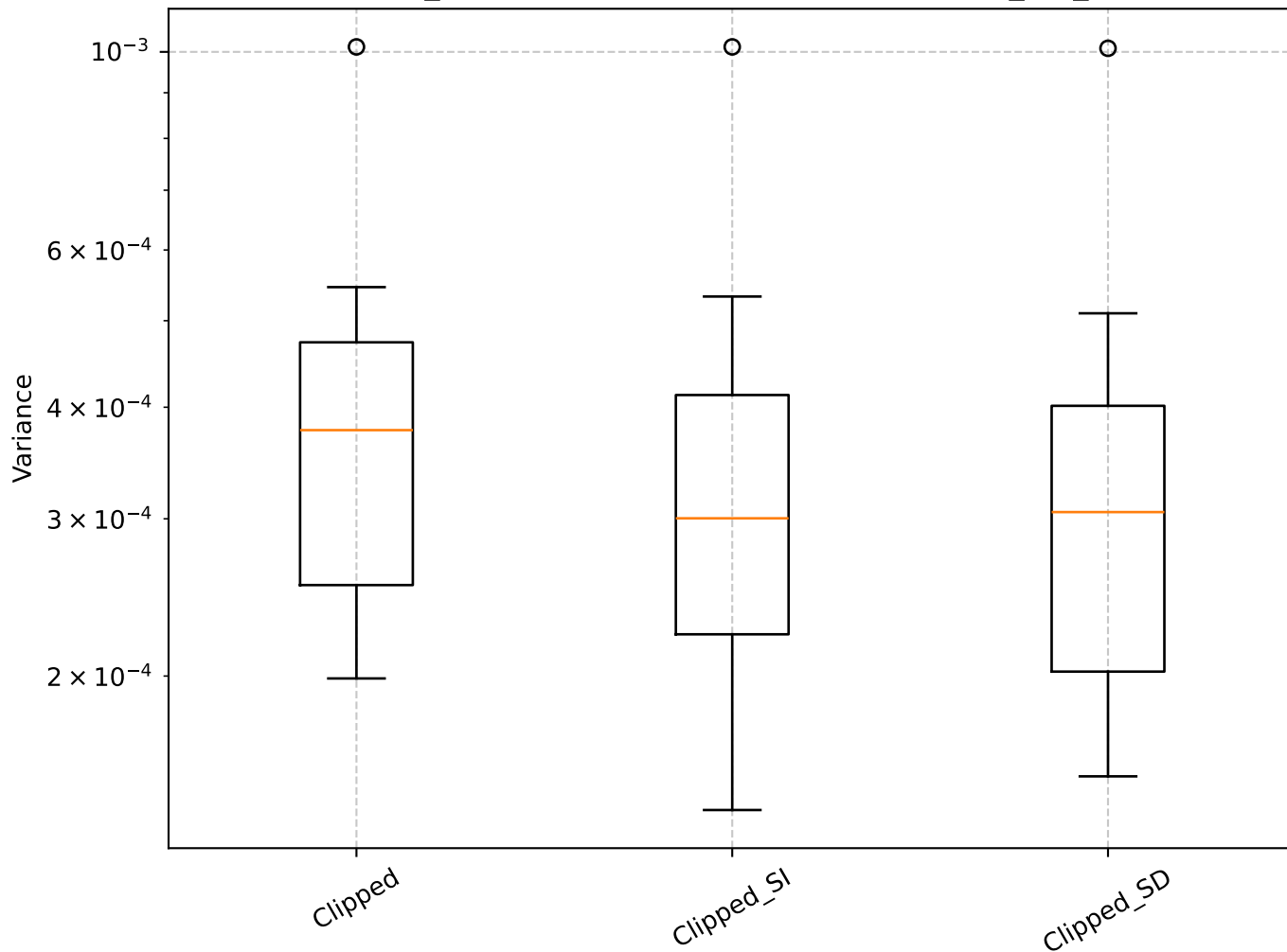
Q=0.73, len_rolling=100: Shrinkage Box Plot - min_var_, Clipped
