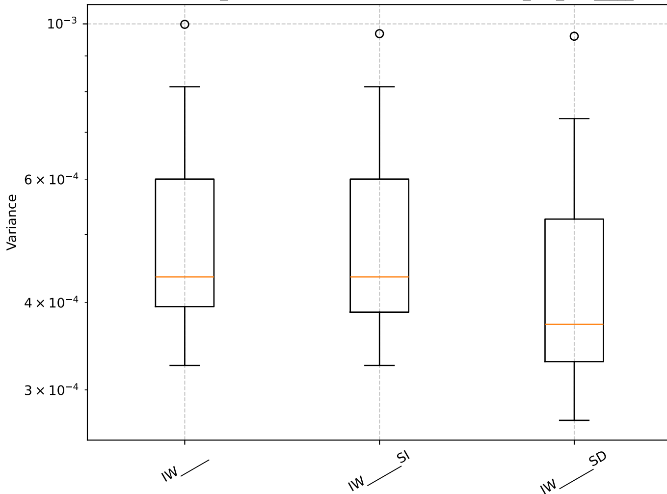
Q=0.73, len_rolling=100: Shrinkage Box Plot - min_var_, IW_____
