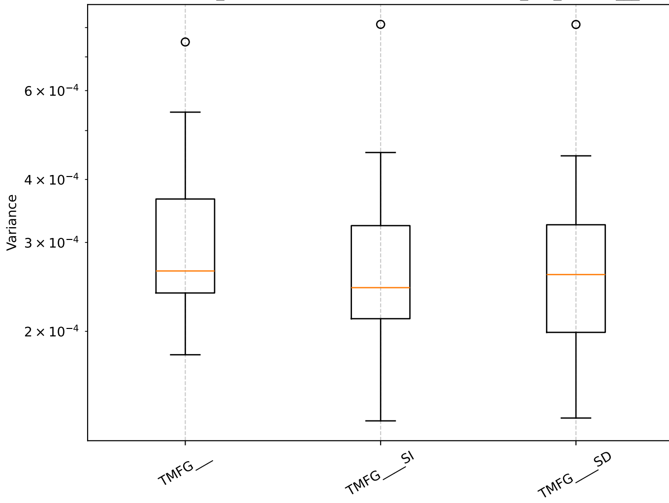
Q=0.75, len_rolling=100: Shrinkage Box Plot - min_var_, TMFG__
