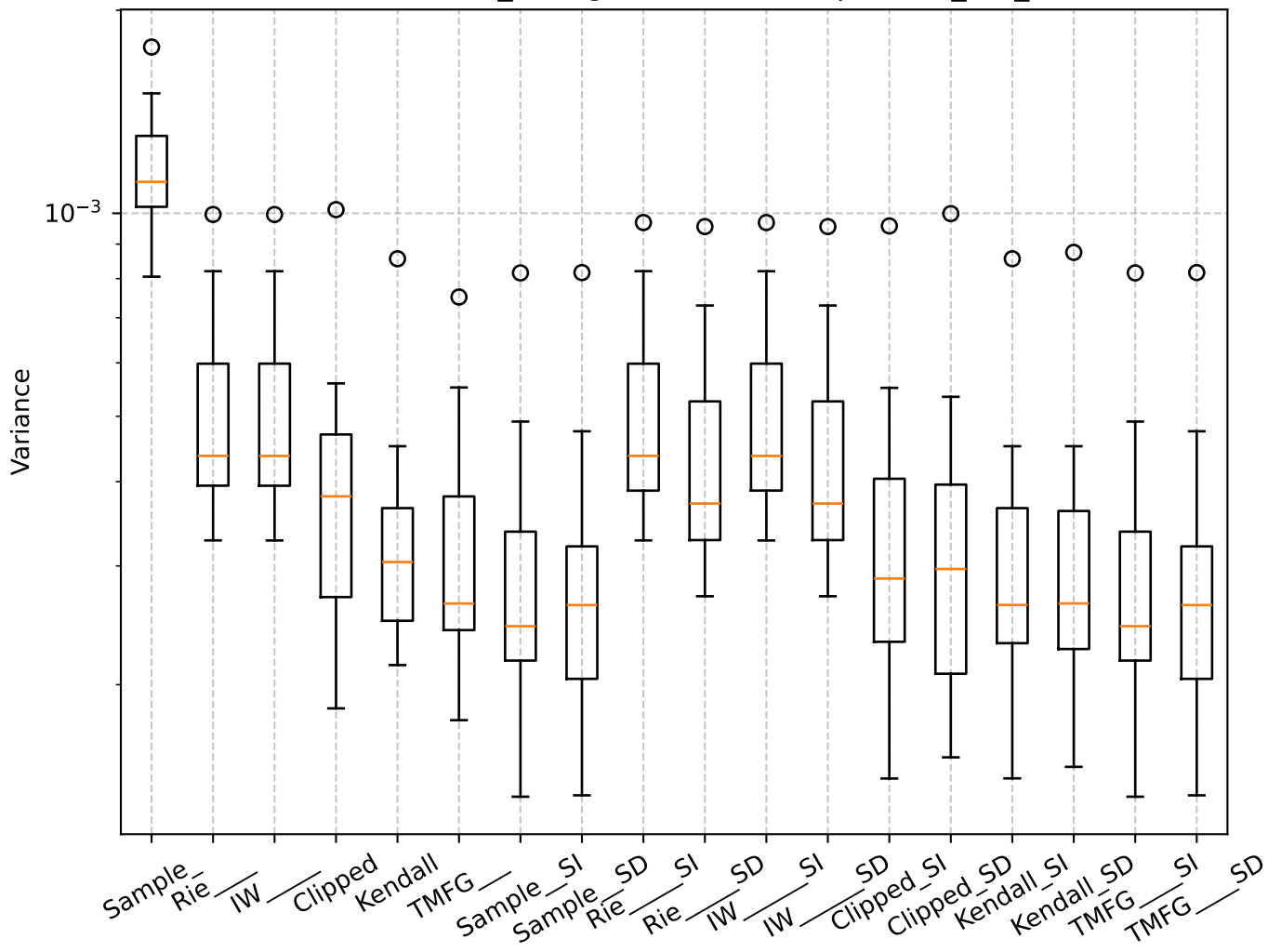
Q=0.78, len_rolling=100: Box Plot per min_var_
