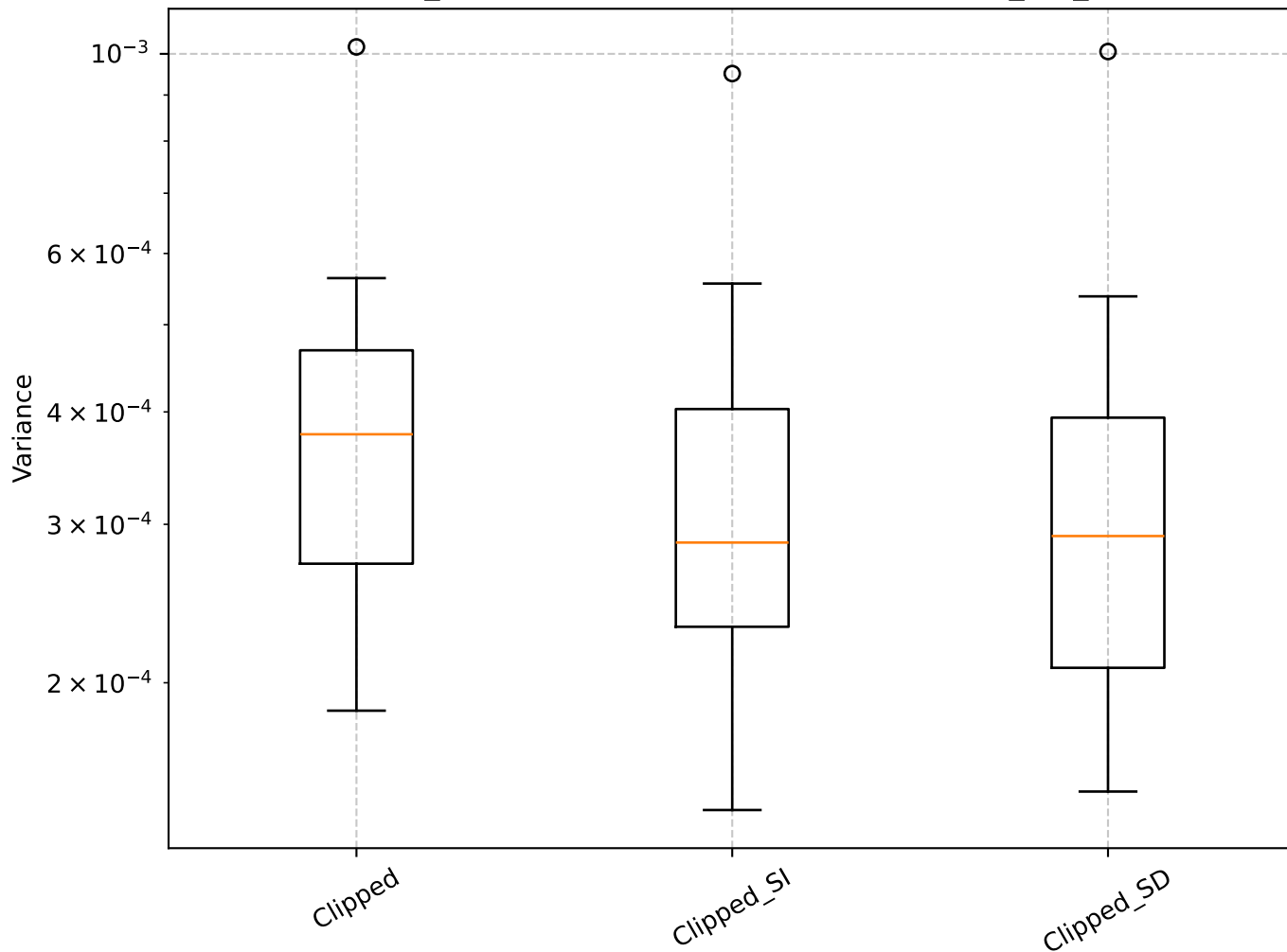
Q=0.80, len_rolling=100: Shrinkage Box Plot - min_var_, Clipped
