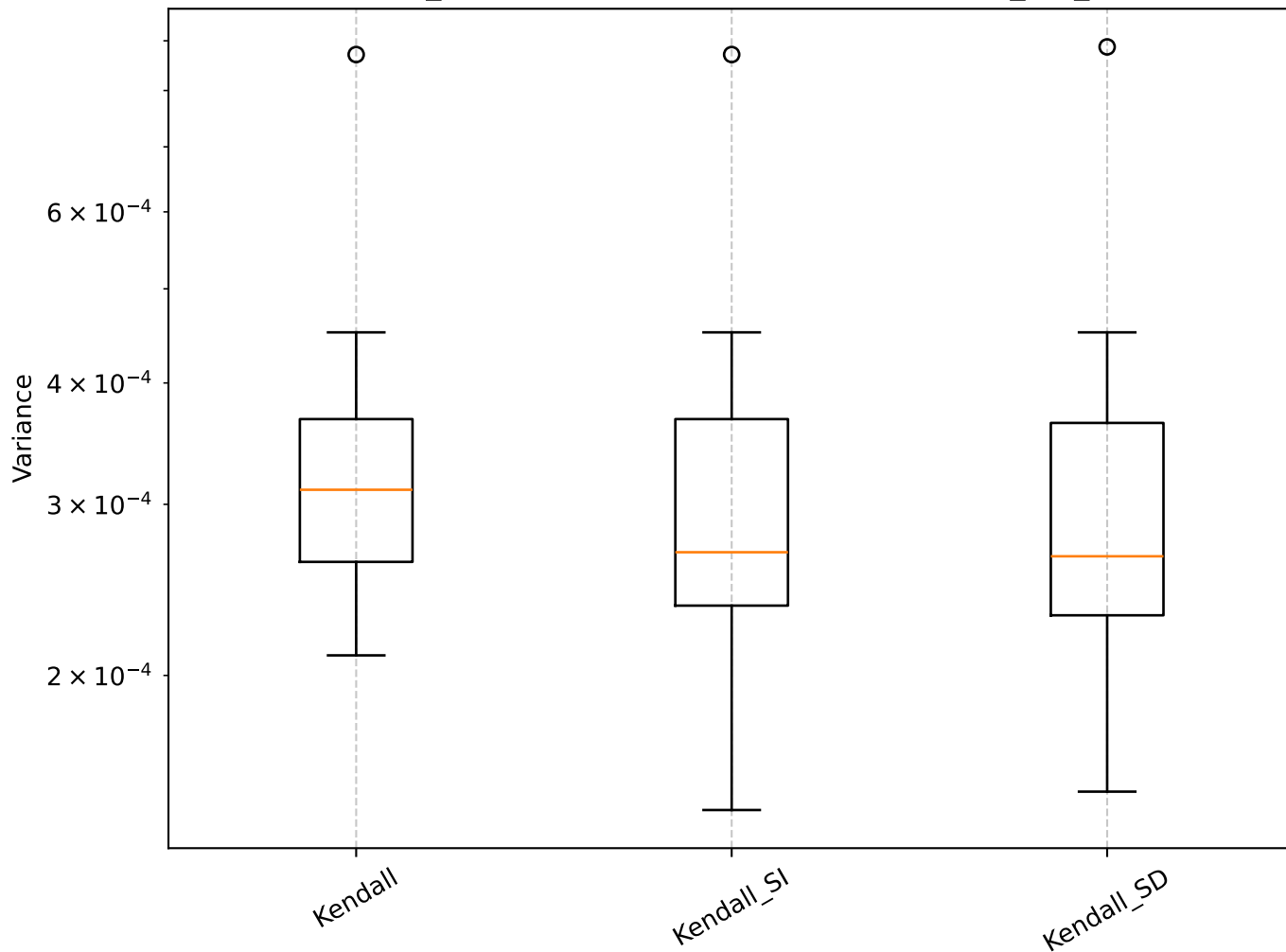
Q=0.82, len_rolling=100: Shrinkage Box Plot - min_var_, Kendall
