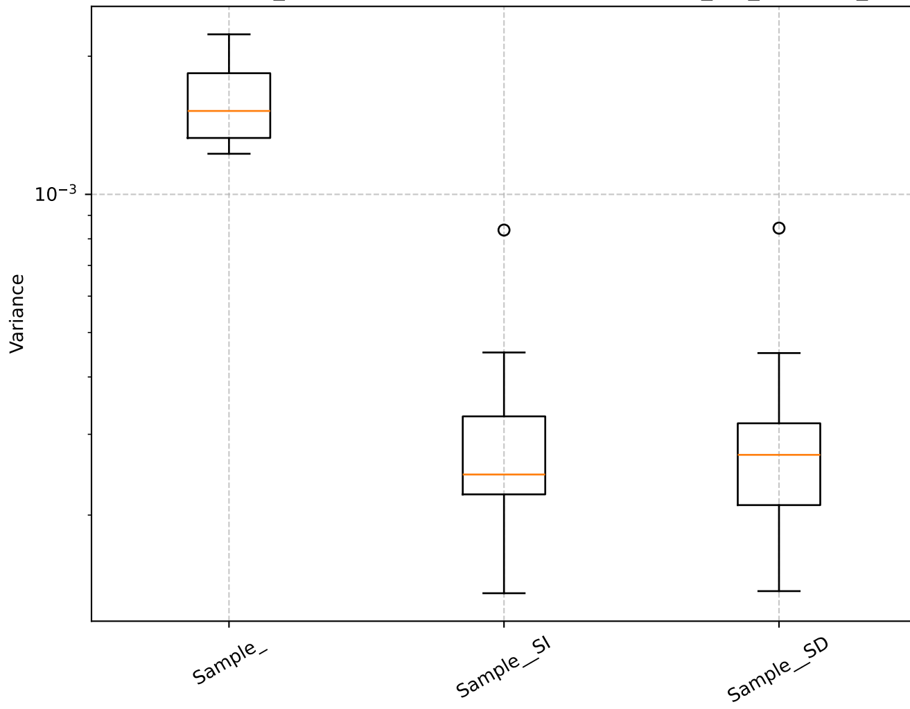
Q=0.83, len_rolling=100: Shrinkage Box Plot - min_var_, Sample_
