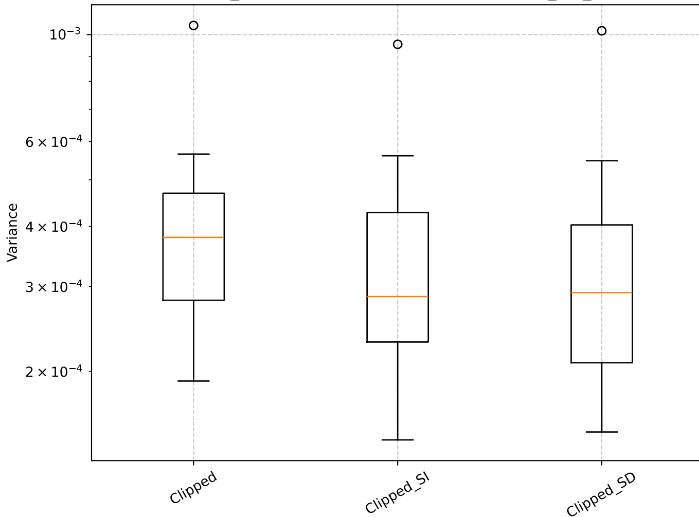
Q=0.85, len_rolling=100: Shrinkage Box Plot - min_var_, Clipped
