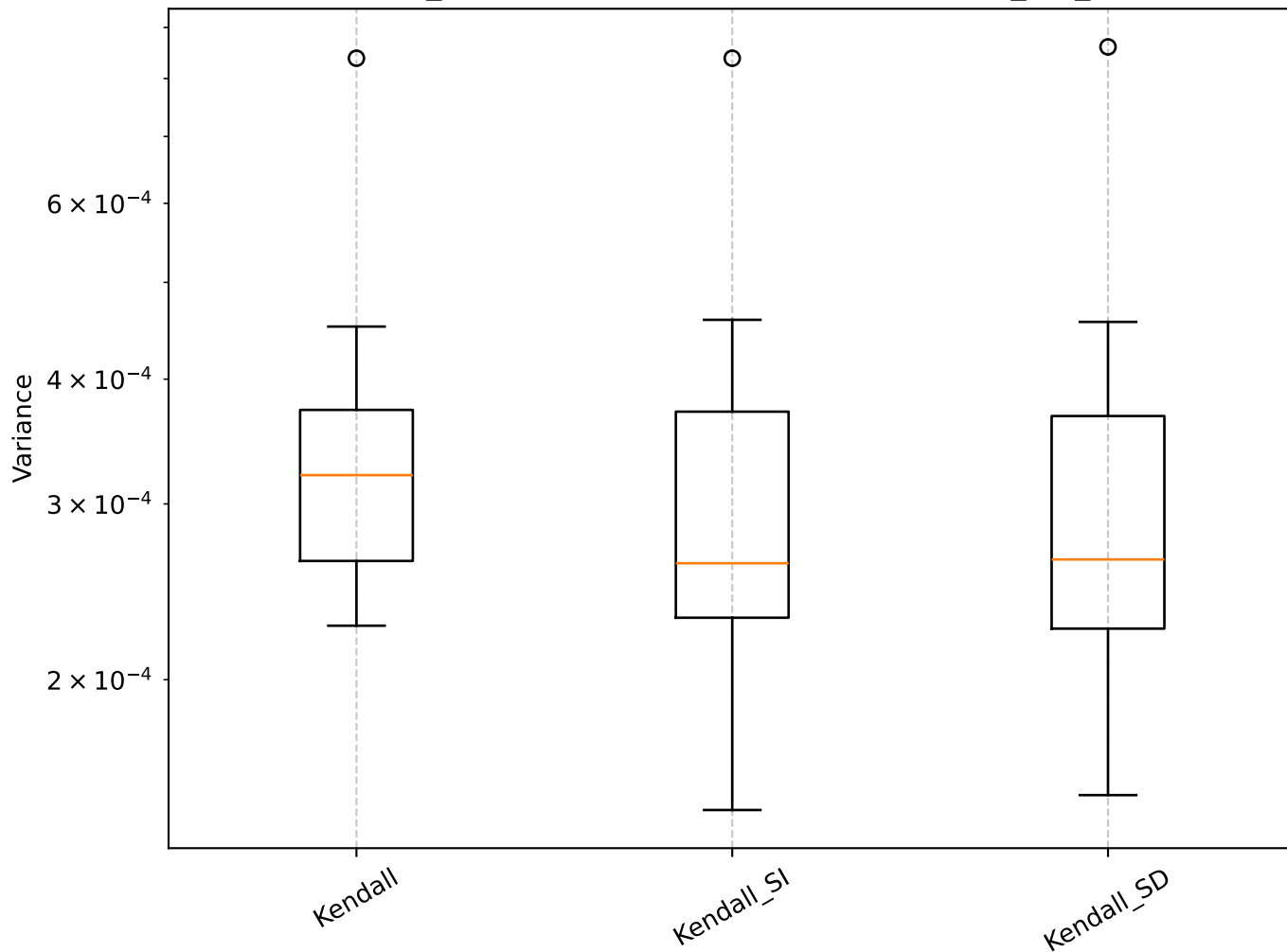
Q=0.89, len_rolling=100: Shrinkage Box Plot - min_var_, Kendall
