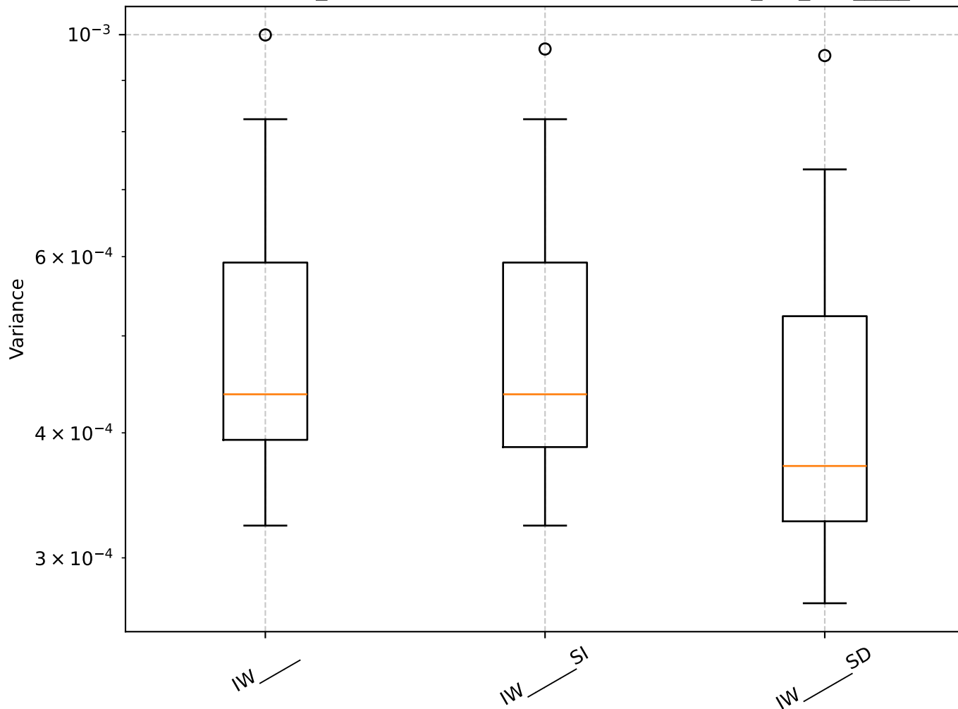
Q=0.93, len_rolling=100: Shrinkage Box Plot - min_var_, IW_____
