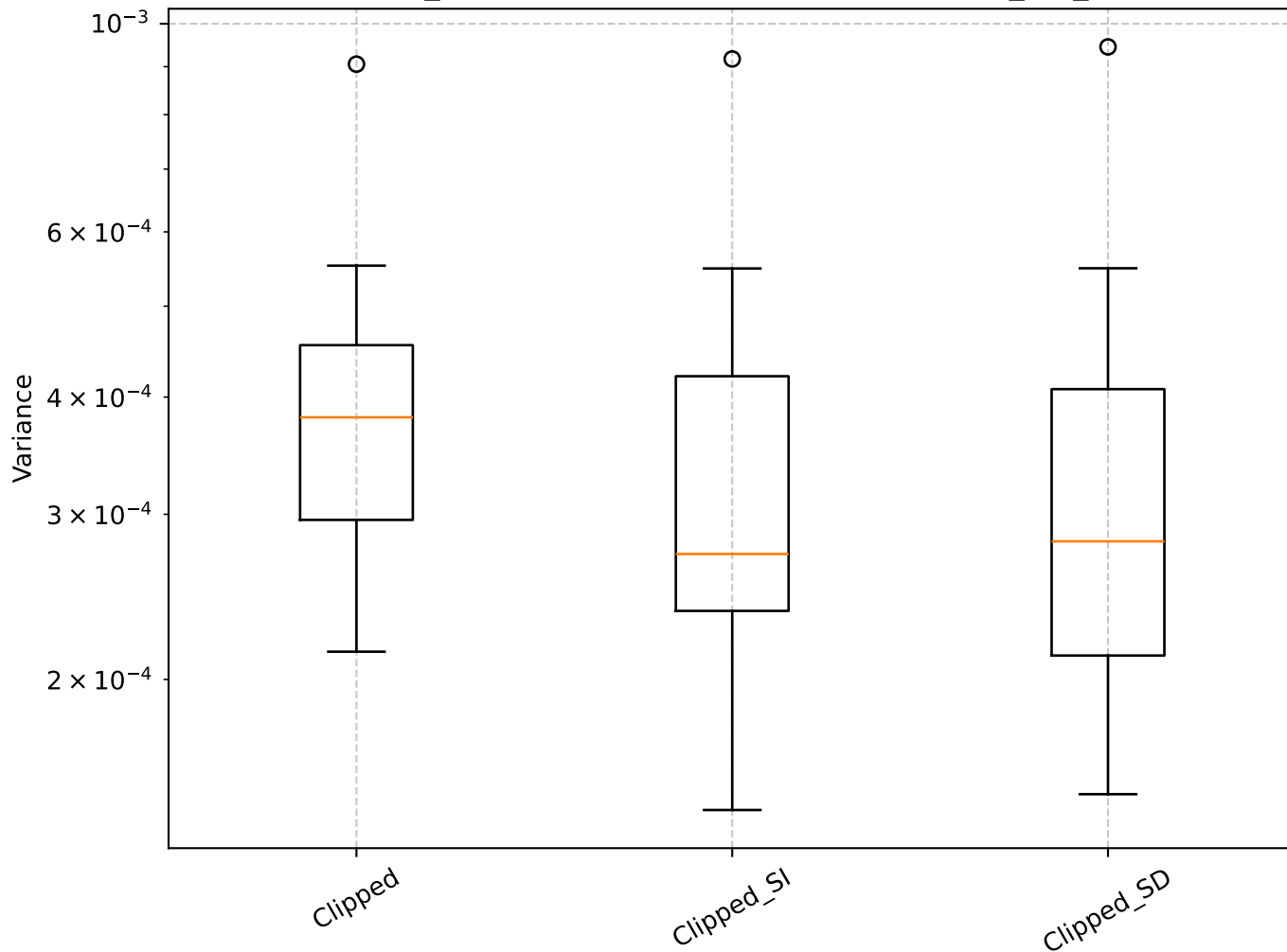
Q=0.98, len_rolling=100: Shrinkage Box Plot - min_var_, Clipped
