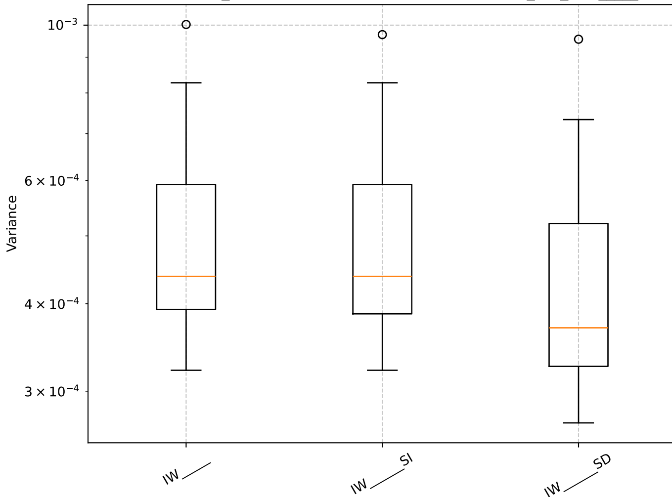
Q=0.98, len_rolling=100: Shrinkage Box Plot - min_var_, IW_____
