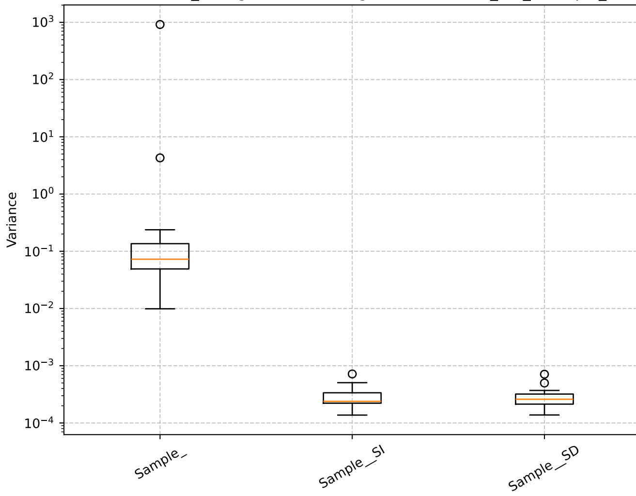
Q=1.05, len_rolling=100: Shrinkage Box Plot - min_var_, Sample_
