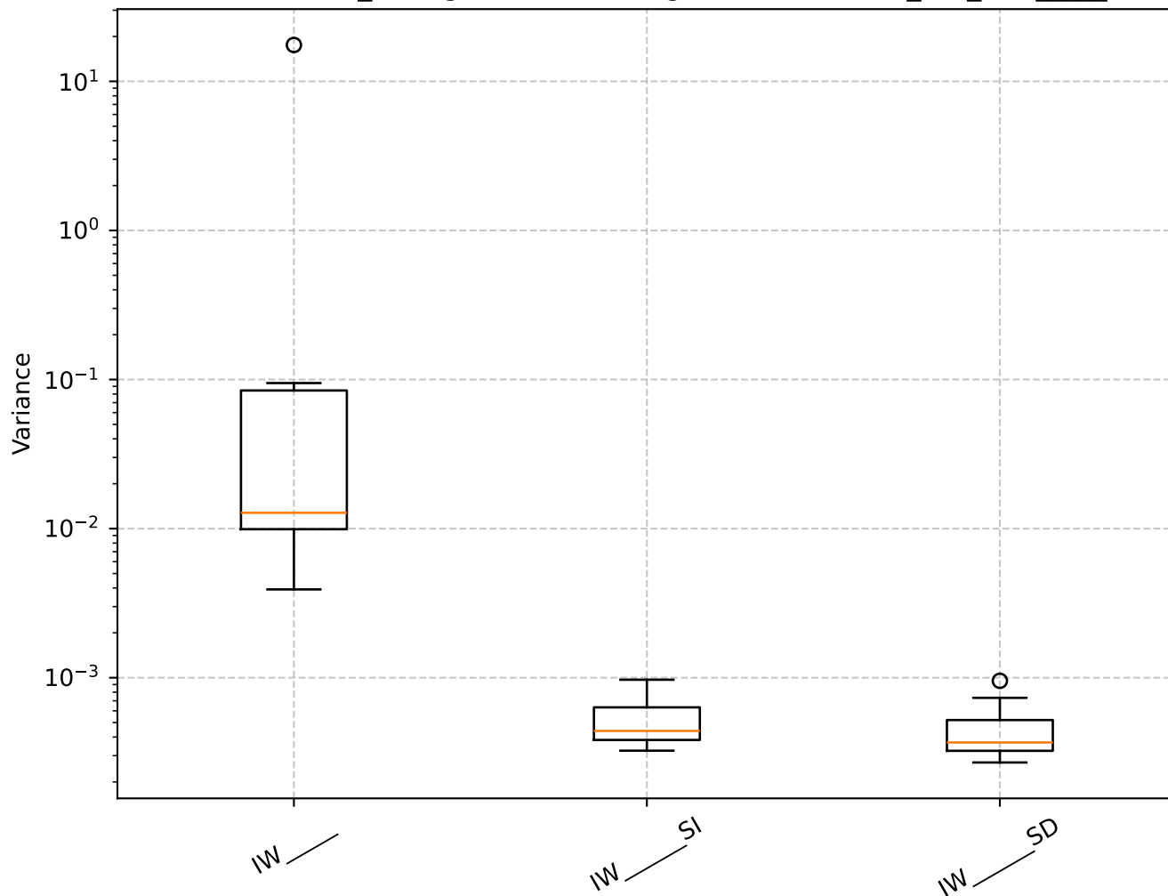
Q=1.11, len_rolling=100: Shrinkage Box Plot - min_var_, IW_____
