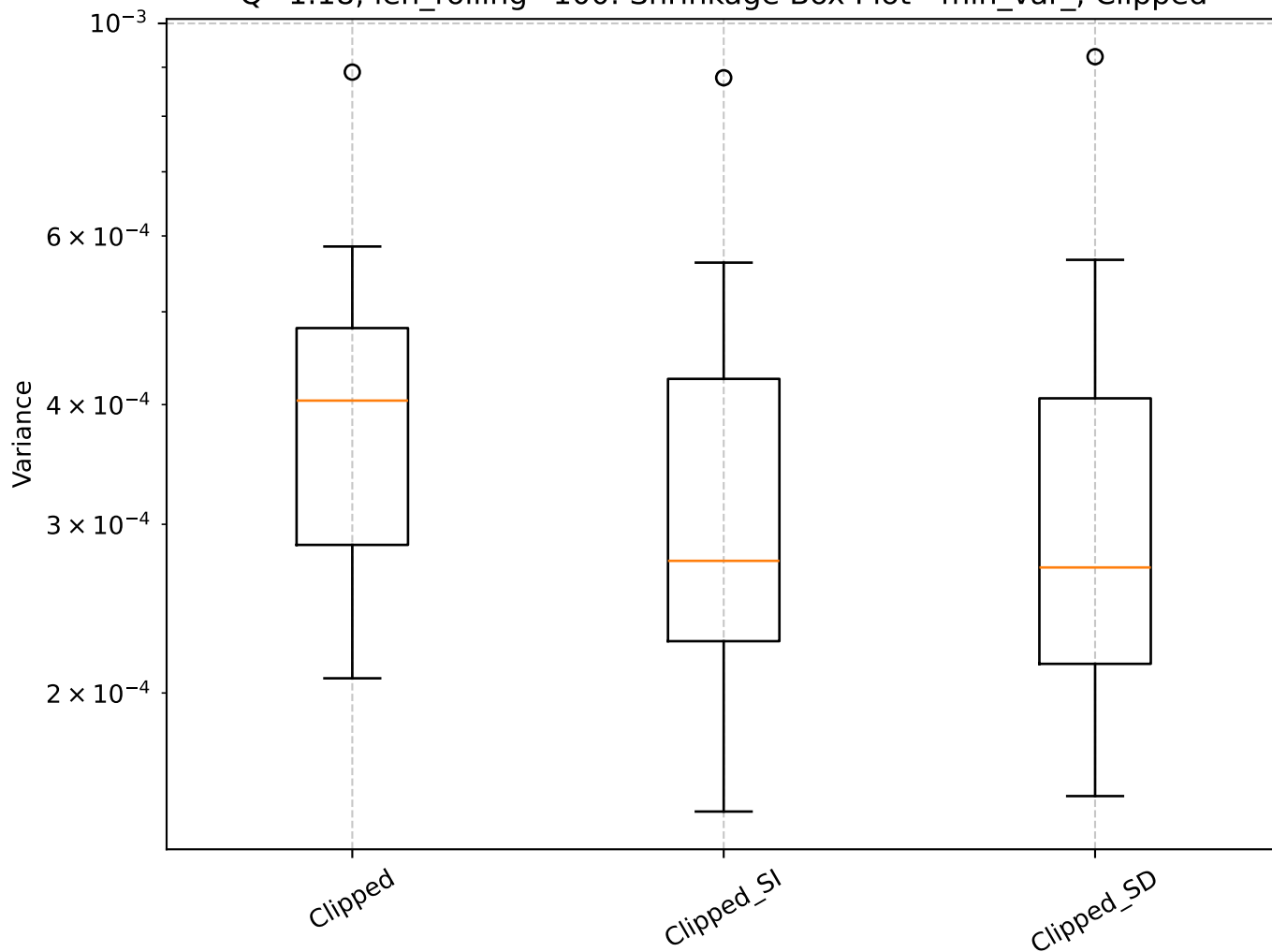
Q=1.18, len_rolling=100: Shrinkage Box Plot - min_var_, Clipped
