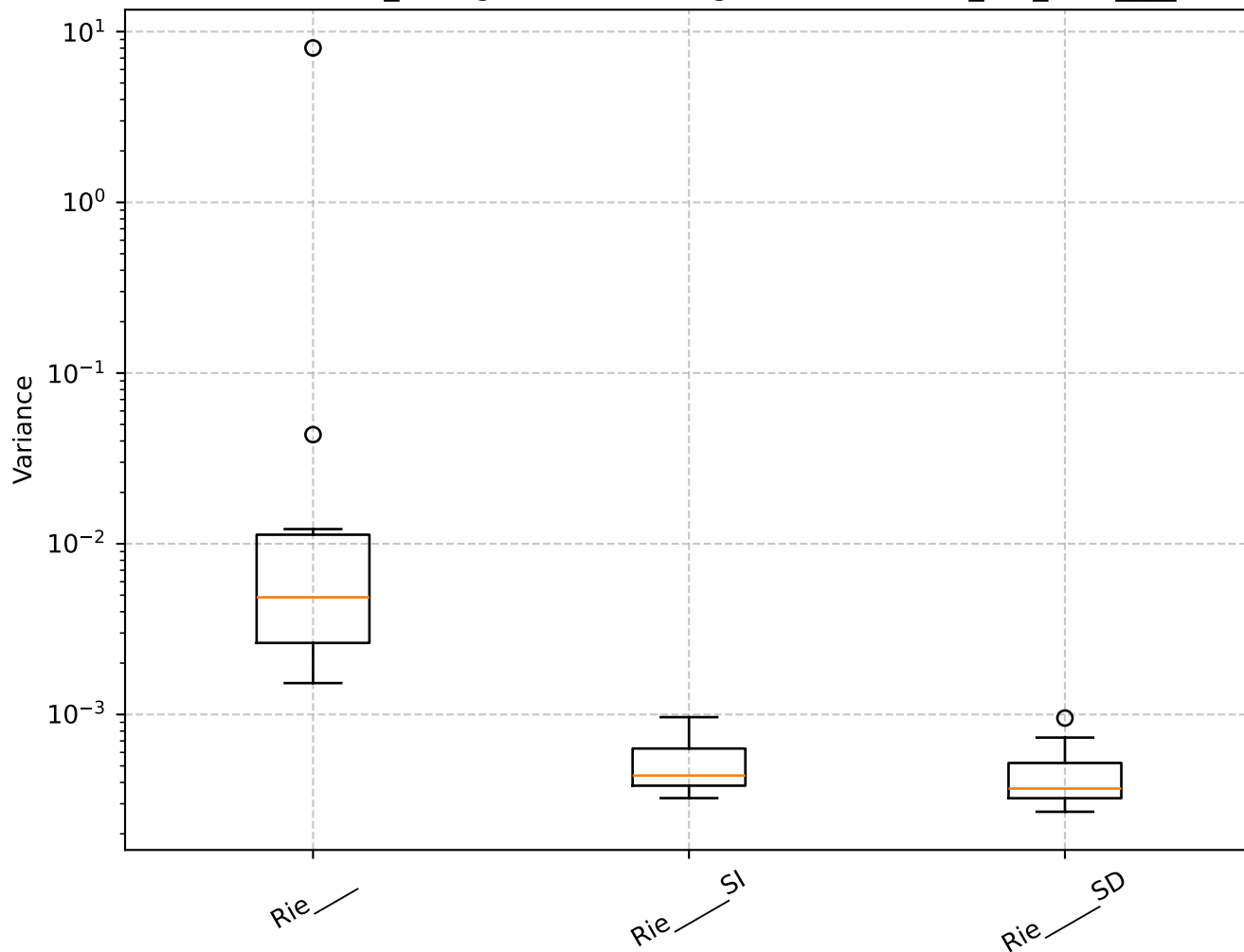
Q=1.18, len_rolling=100: Shrinkage Box Plot - min_var_, Rie____
