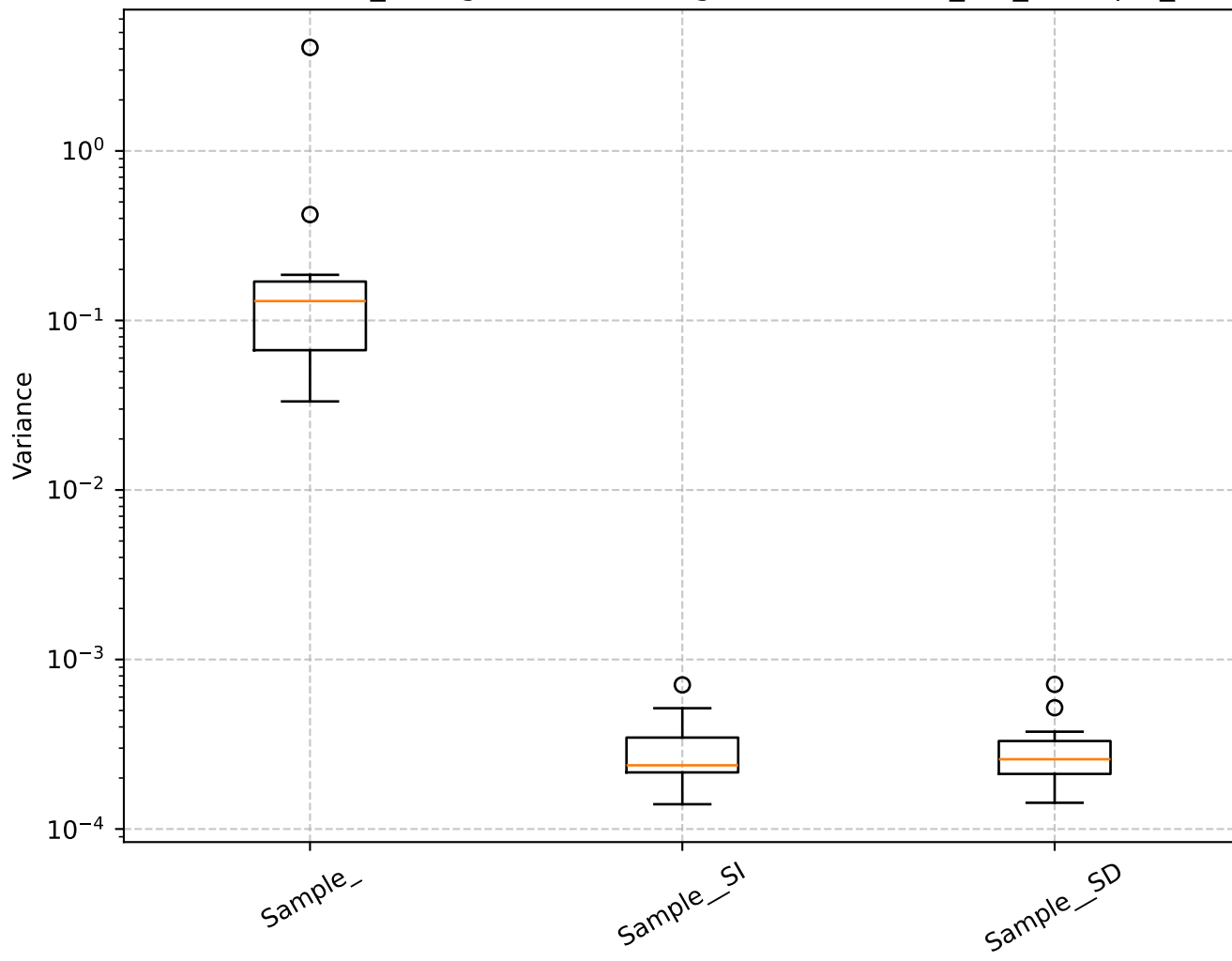
Q=1.18, len_rolling=100: Shrinkage Box Plot - min_var_, Sample_
