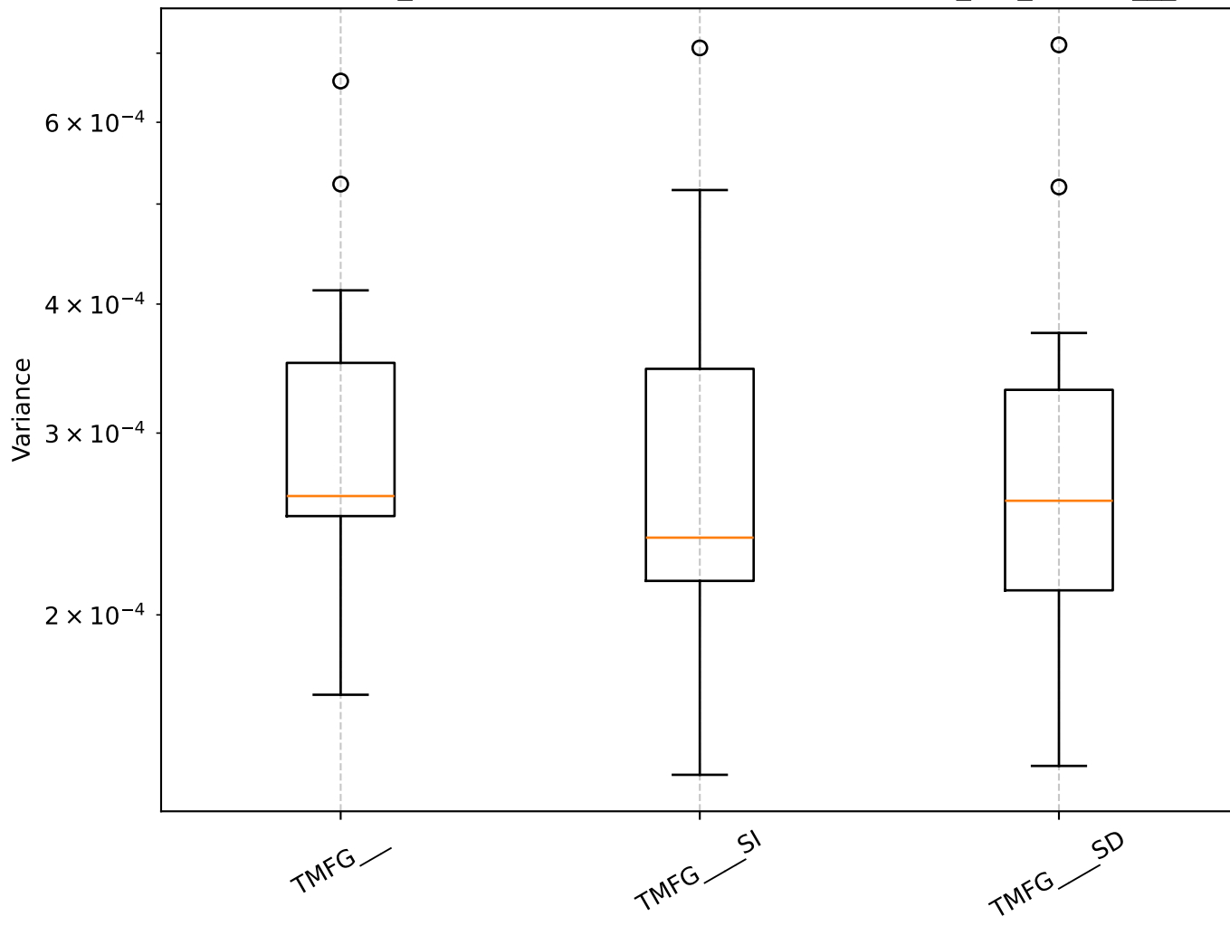
Q=1.18, len_rolling=100: Shrinkage Box Plot - min_var_, TMFG__
