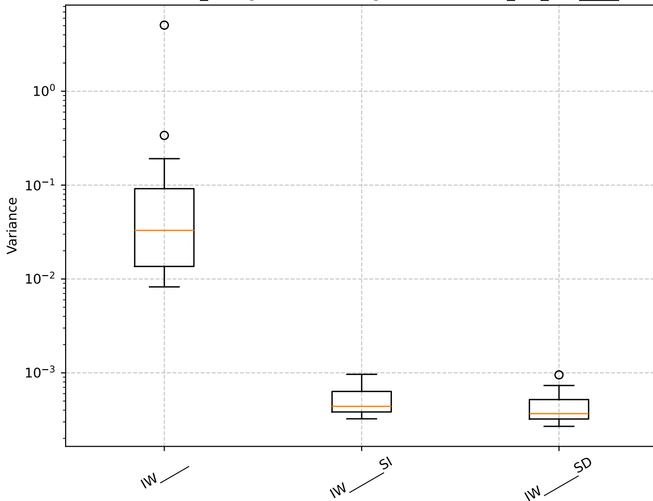
Q=1.21, len_rolling=100: Shrinkage Box Plot - min_var_, IW_____
