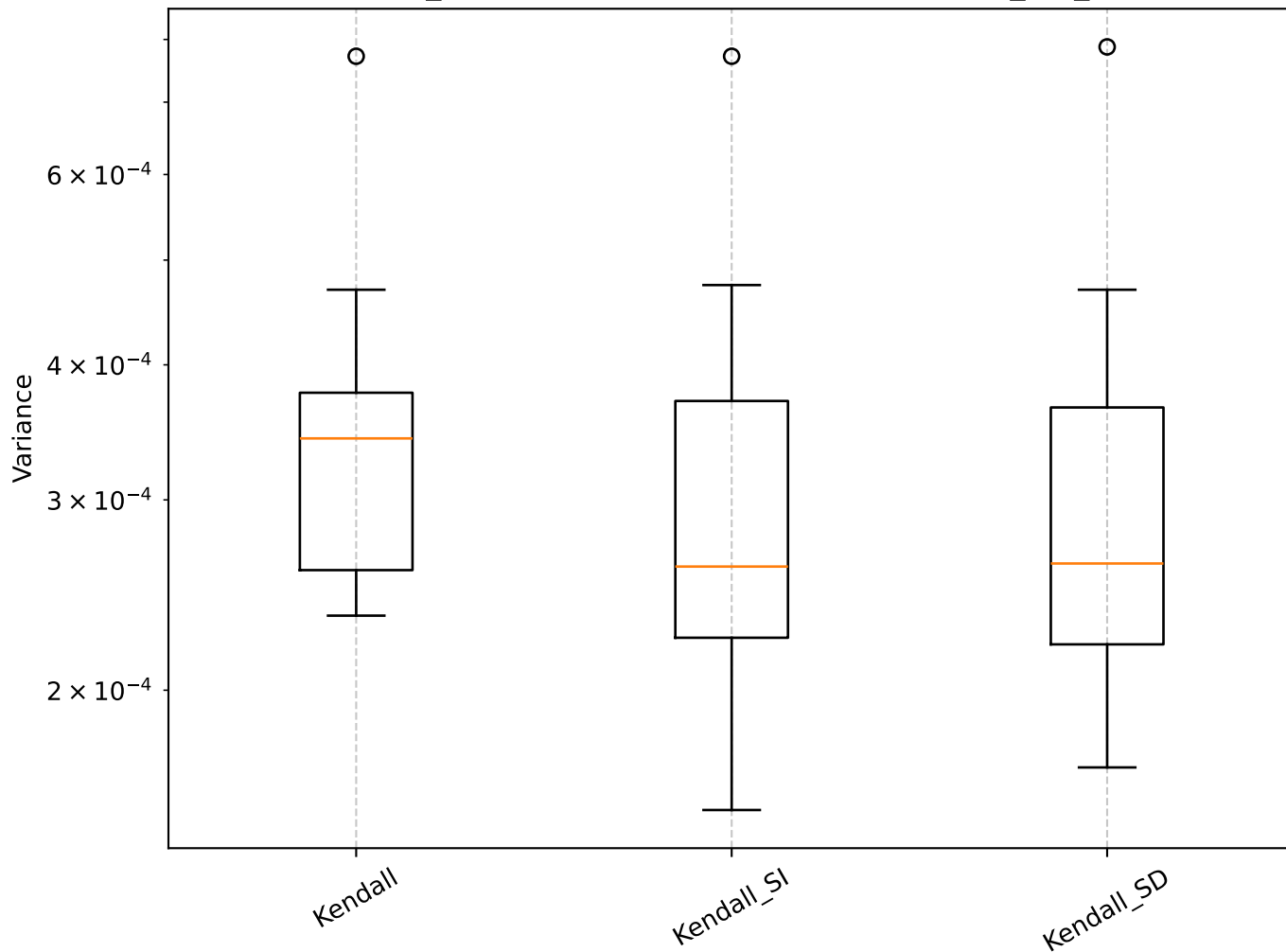
Q=1.25, len_rolling=100: Shrinkage Box Plot - min_var_, Kendall
