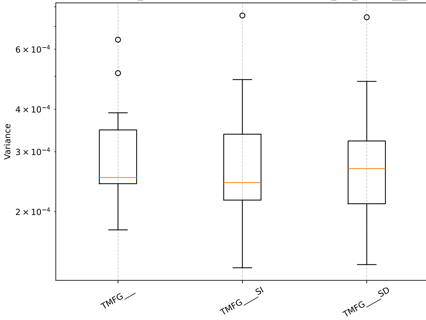
Q=1.25, len_rolling=100: Shrinkage Box Plot - min_var_, TMFG__
