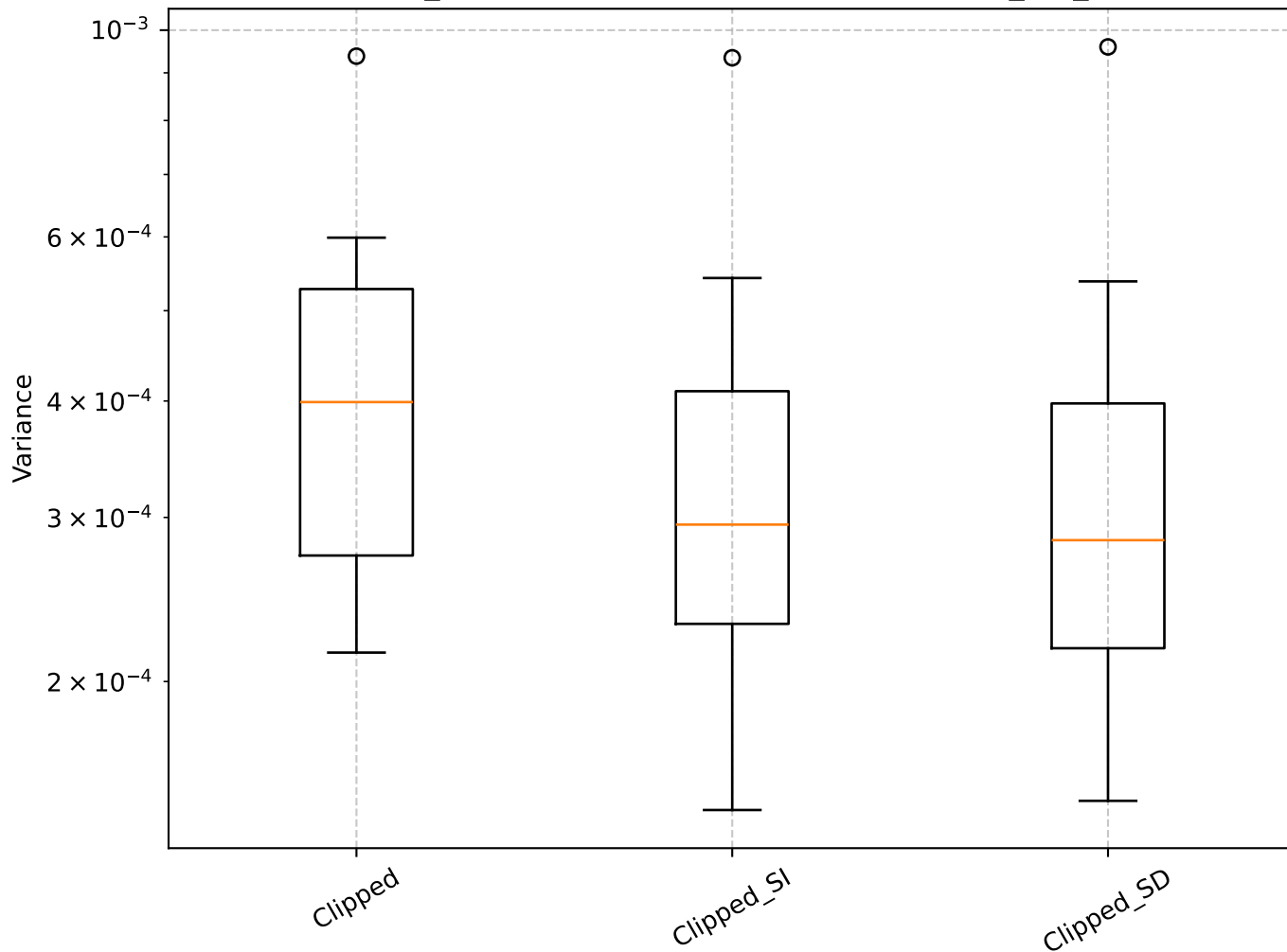
Q=1.33, len_rolling=100: Shrinkage Box Plot - min_var_, Clipped
