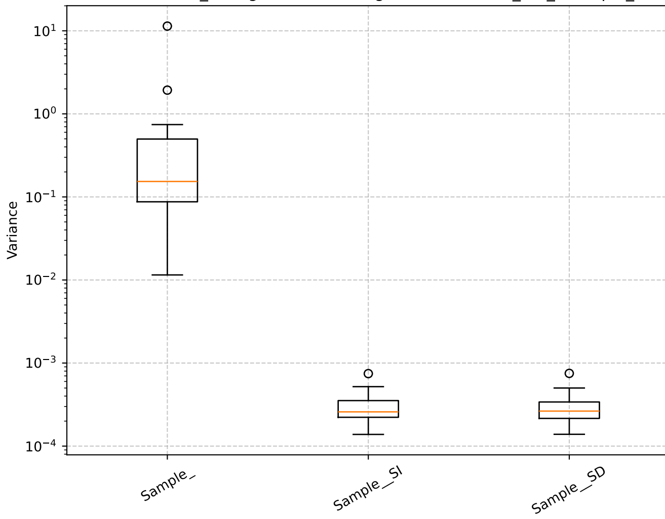
Q=1.38, len_rolling=100: Shrinkage Box Plot - min_var_, Sample_
