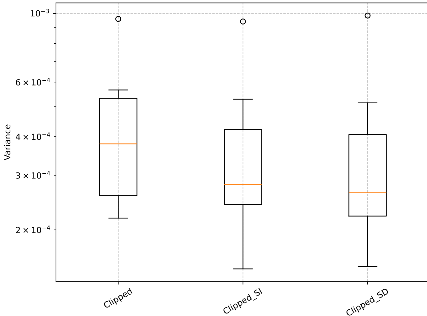
Q=1.54, len_rolling=100: Shrinkage Box Plot - min_var_, Clipped
