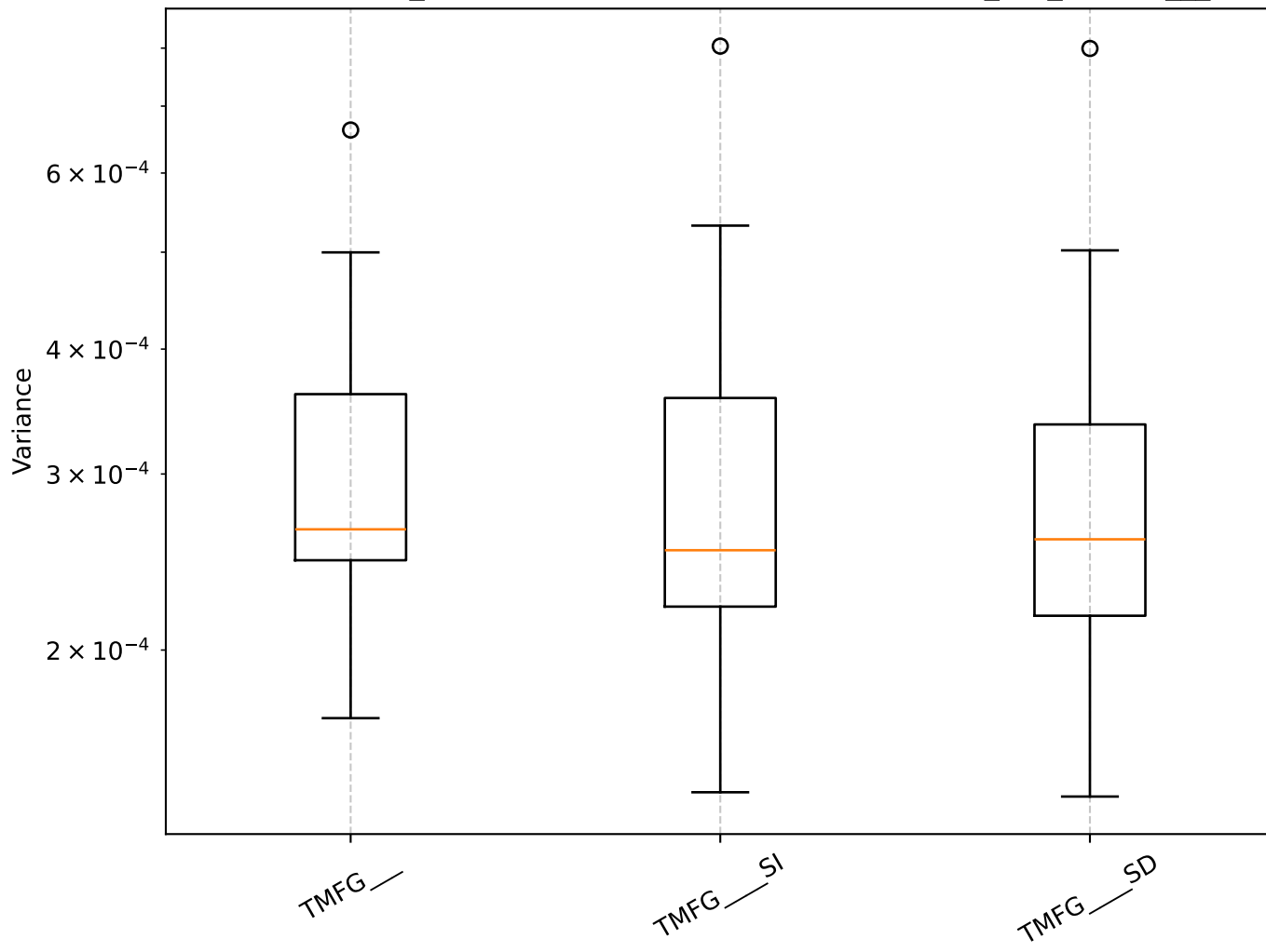
Q=1.54, len_rolling=100: Shrinkage Box Plot - min_var_, TMFG__
