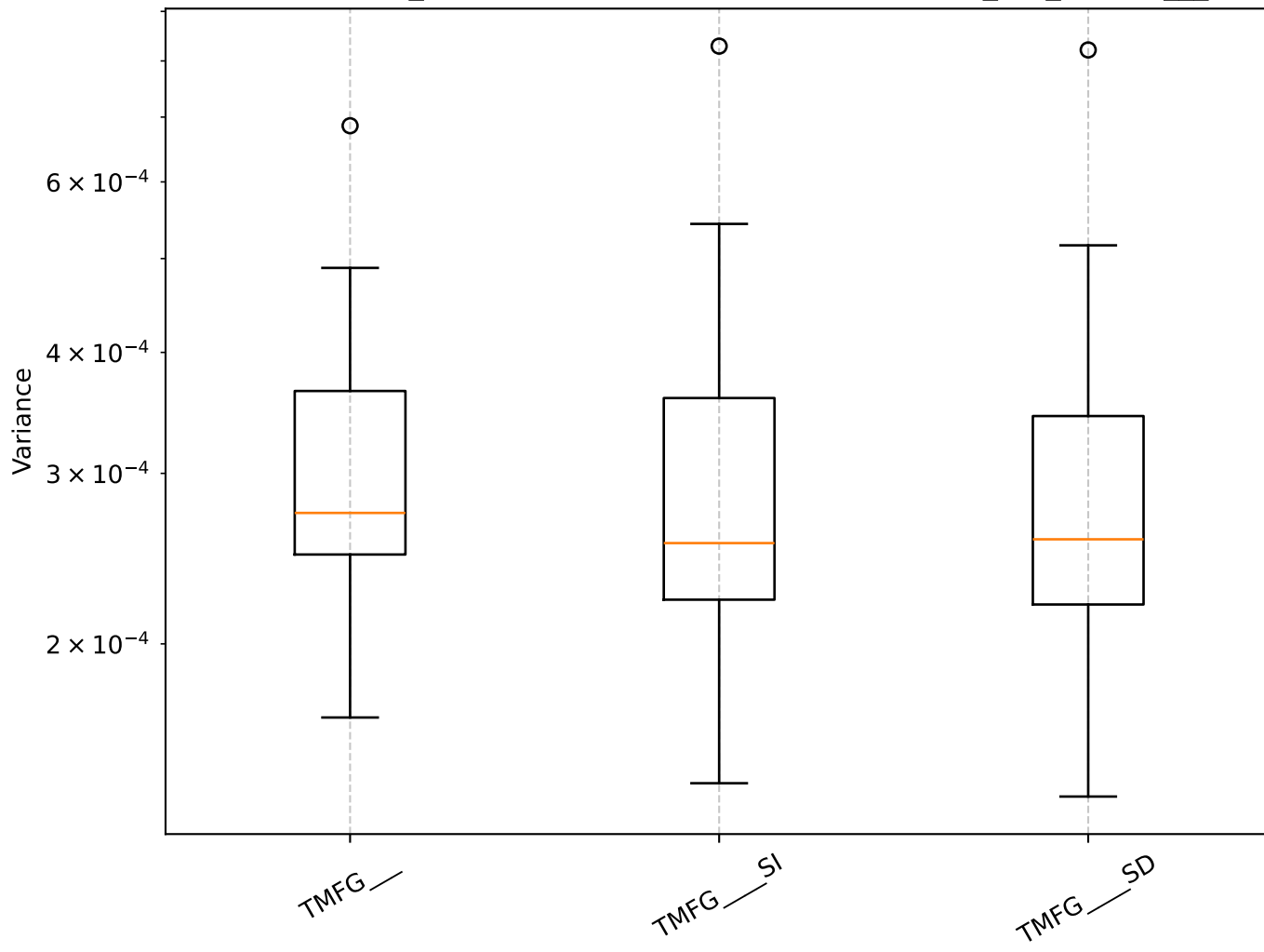
Q=1.67, len_rolling=100: Shrinkage Box Plot - min_var_, TMFG__
