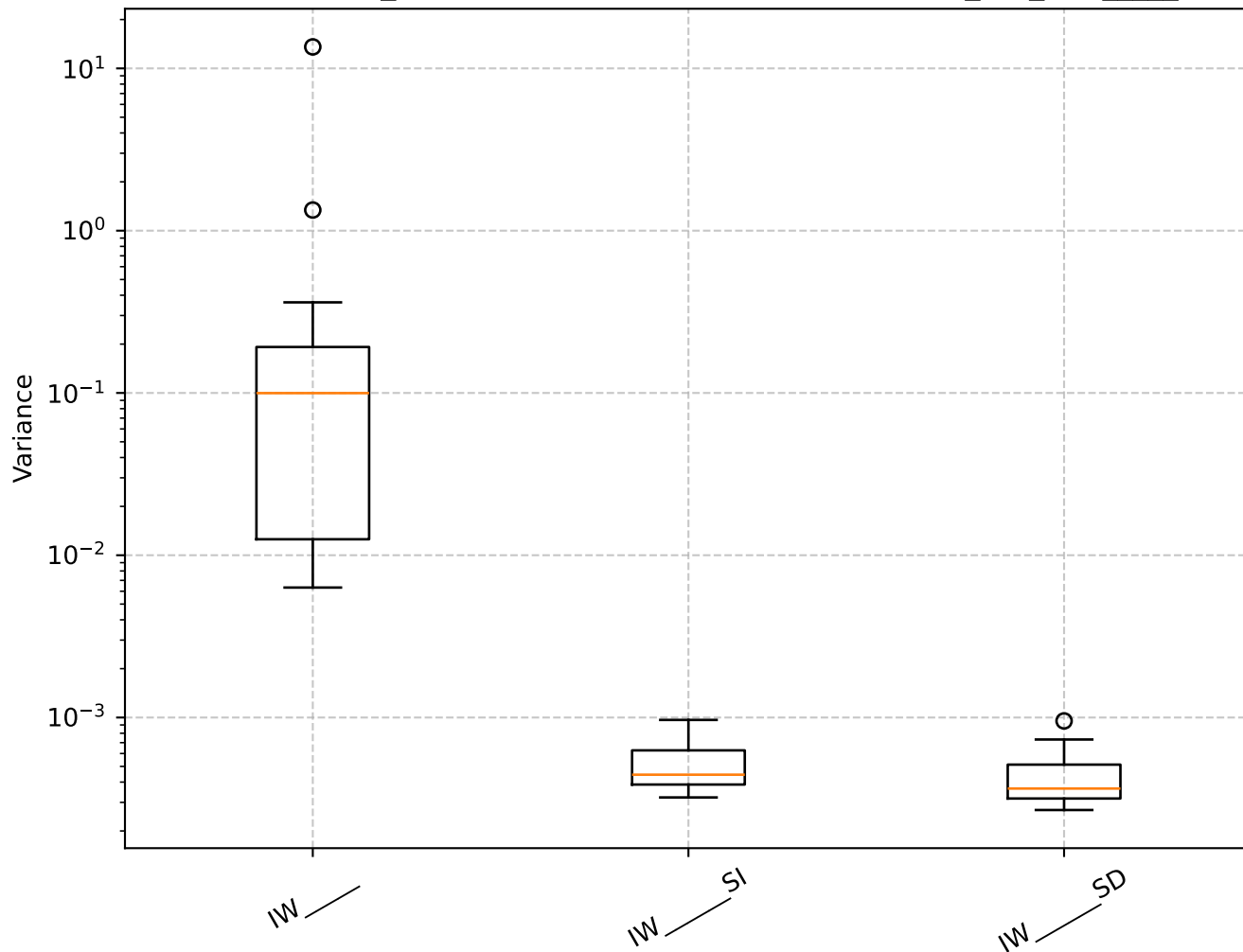
Q=1.75, len_rolling=100: Shrinkage Box Plot - min_var_, IW_____
