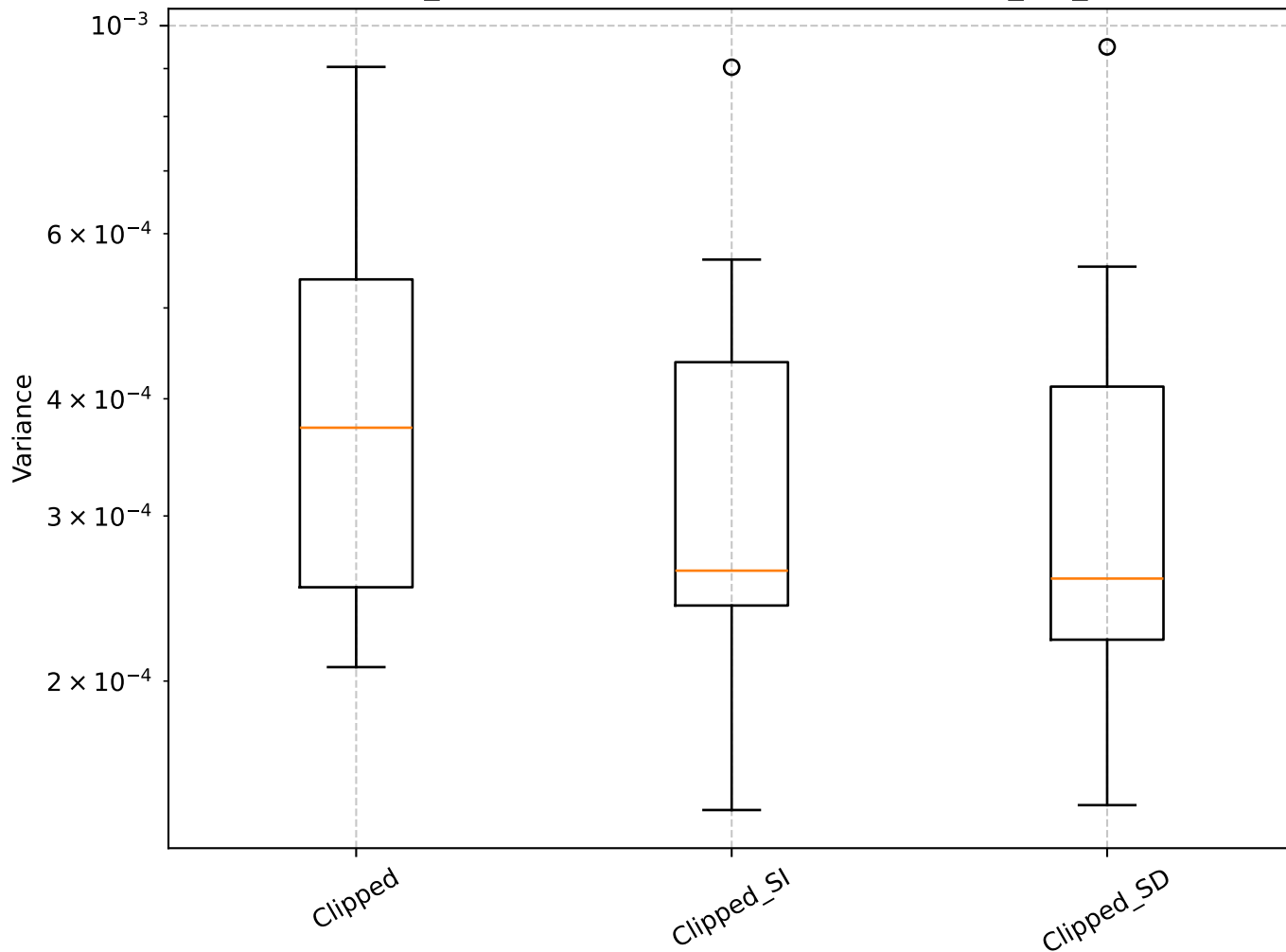
Q=1.83, len_rolling=100: Shrinkage Box Plot - min_var_, Clipped
