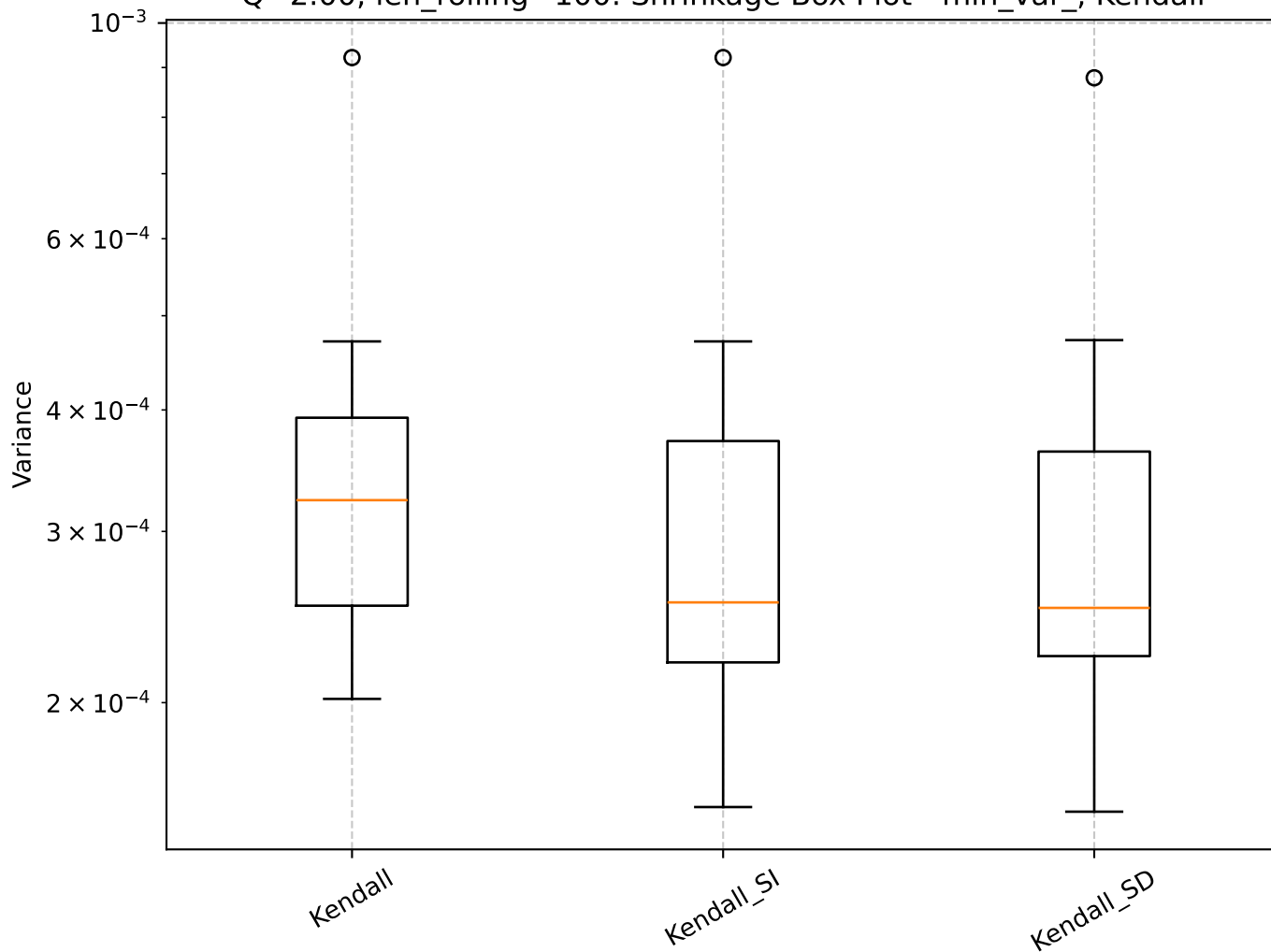
Q=2.00, len_rolling=100: Shrinkage Box Plot - min_var_, Kendall
