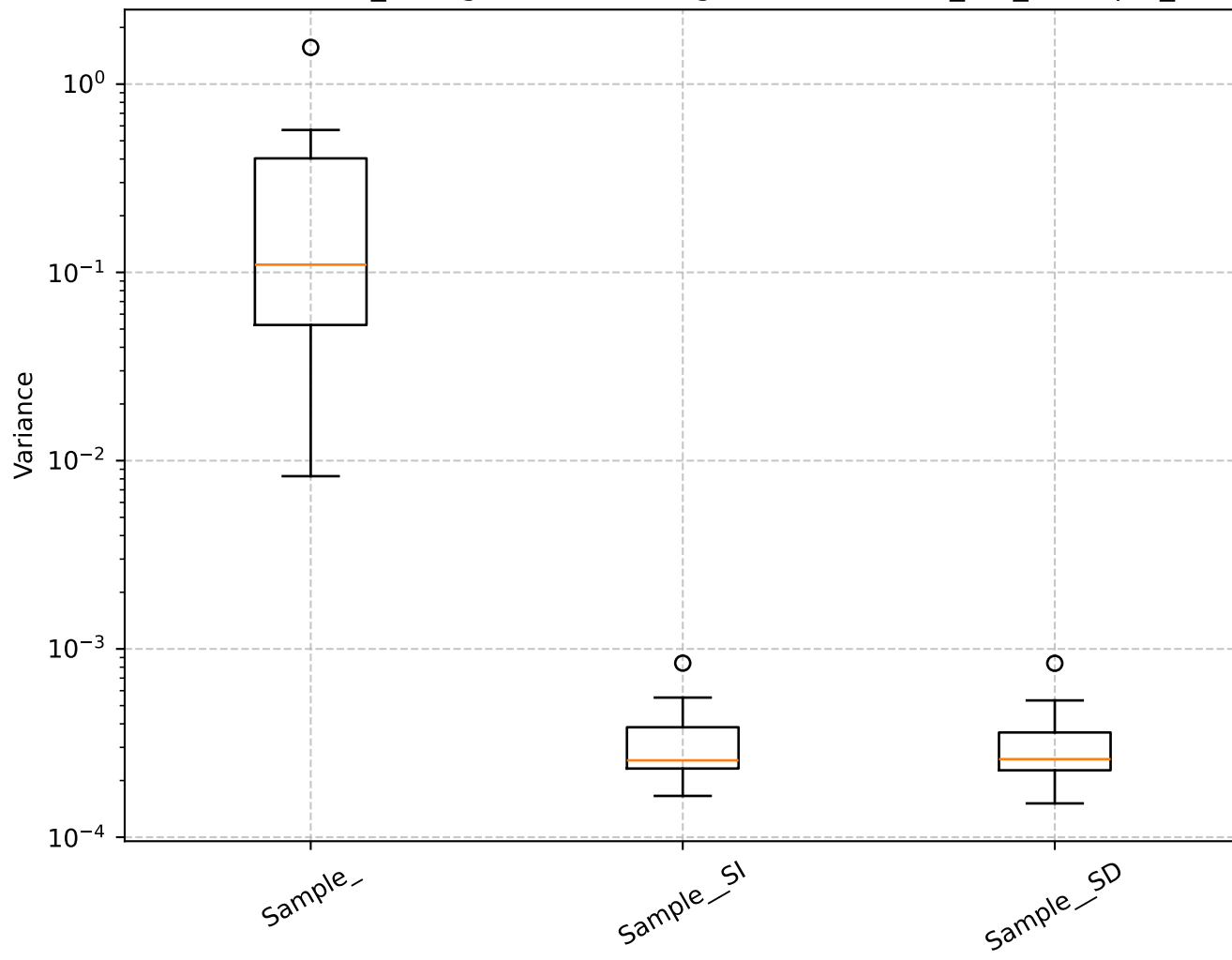
Q=2.88, len_rolling=100: Shrinkage Box Plot - min_var_, Sample_
