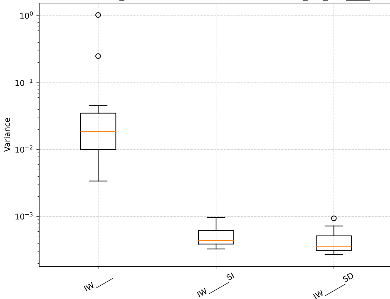
Q=3.10, len_rolling=100: Shrinkage Box Plot - min_var_, IW_____
