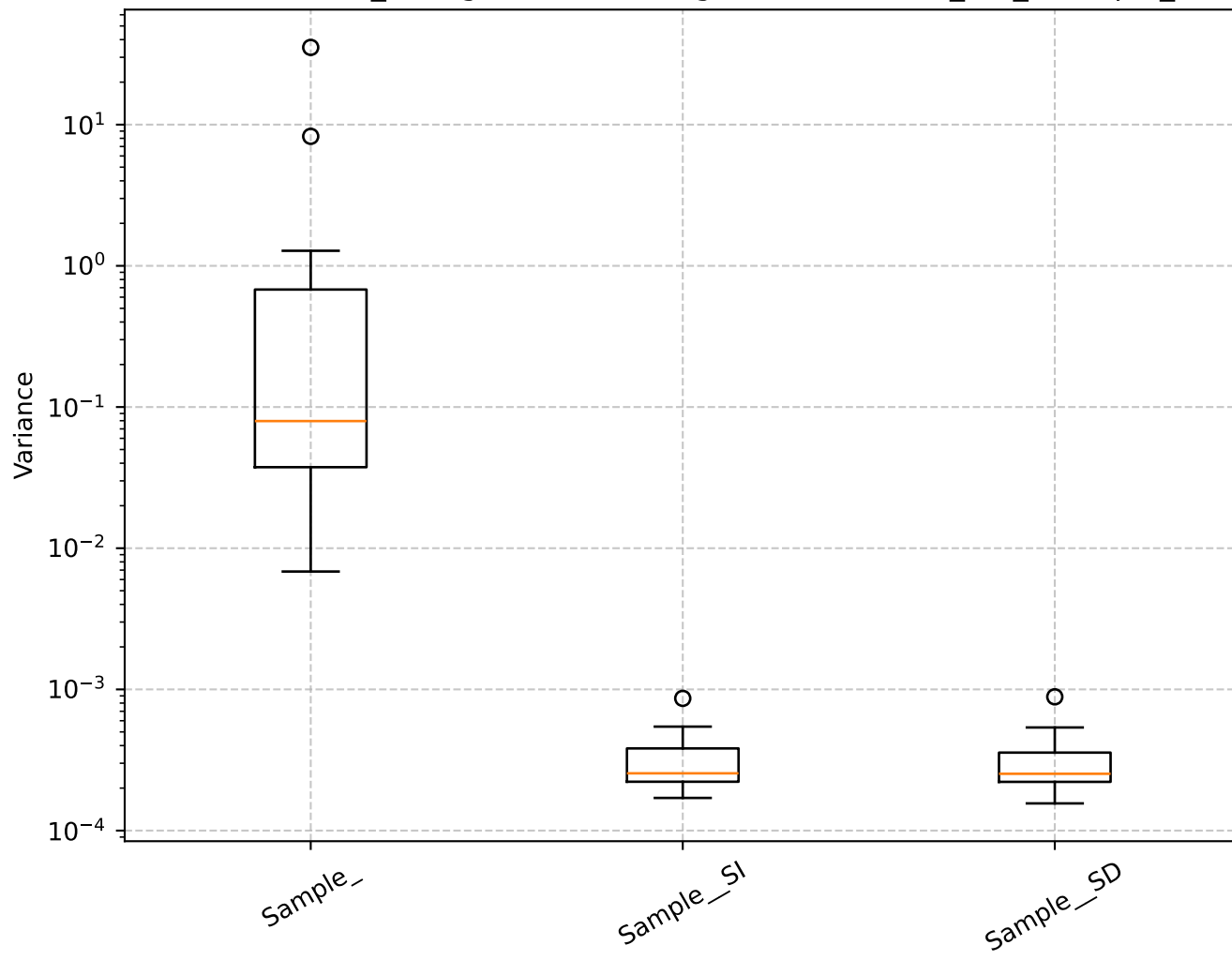
Q=3.10, len_rolling=100: Shrinkage Box Plot - min_var_, Sample_
