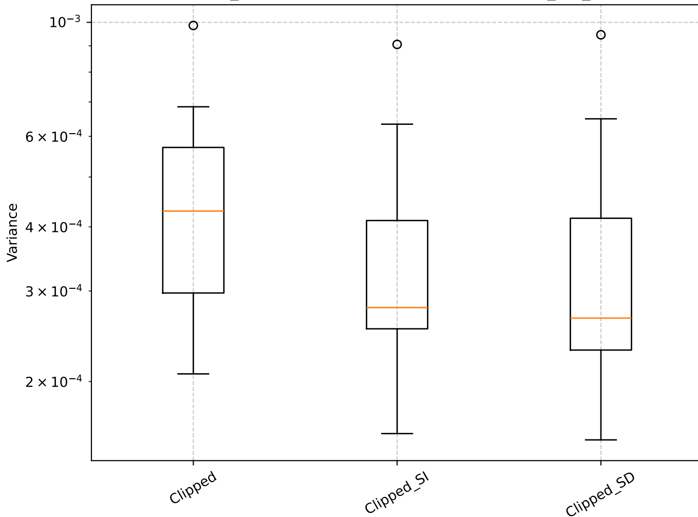
Q=3.33, len_rolling=100: Shrinkage Box Plot - min_var_, Clipped
