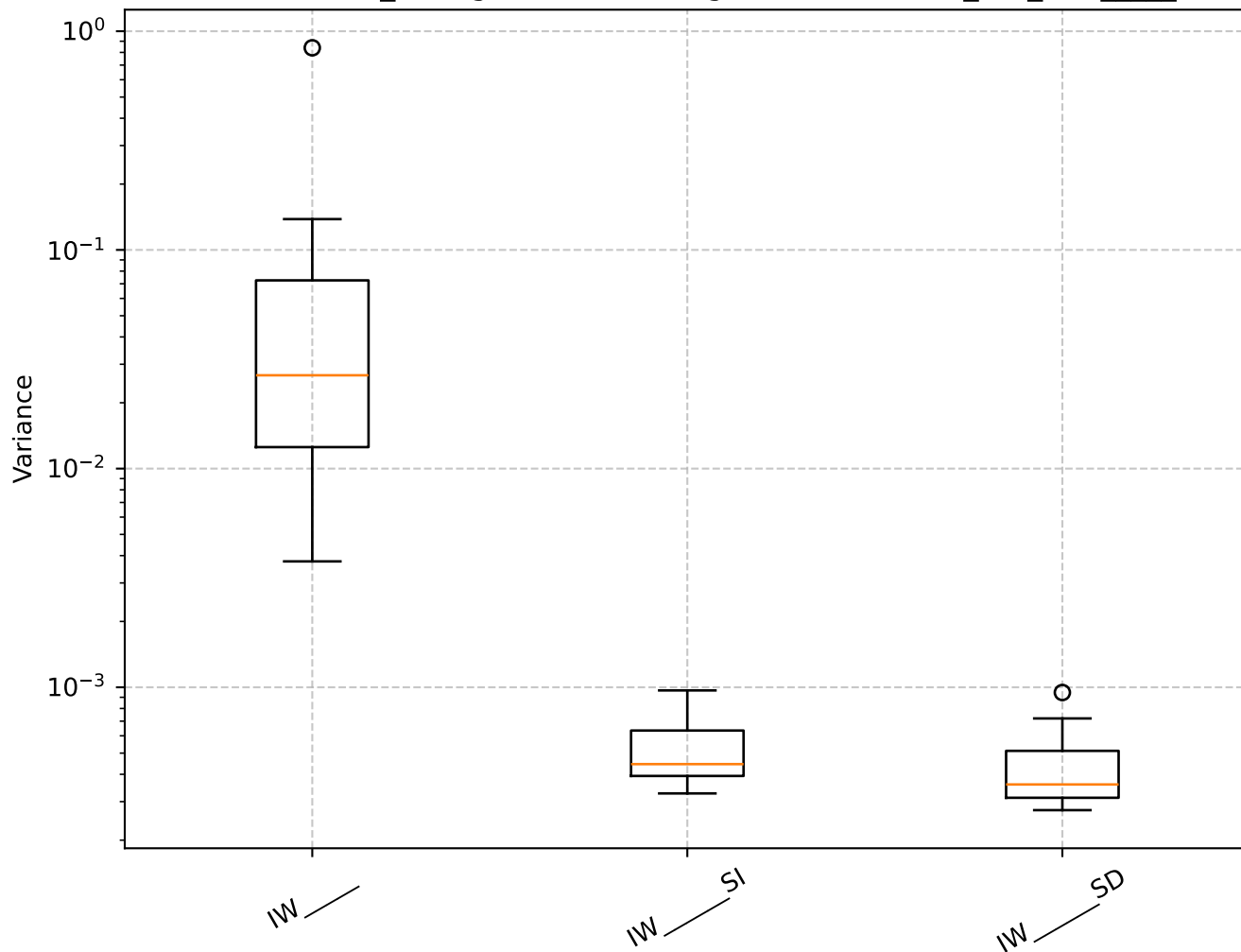
Q=4.00, len_rolling=100: Shrinkage Box Plot - min_var_, IW_____
