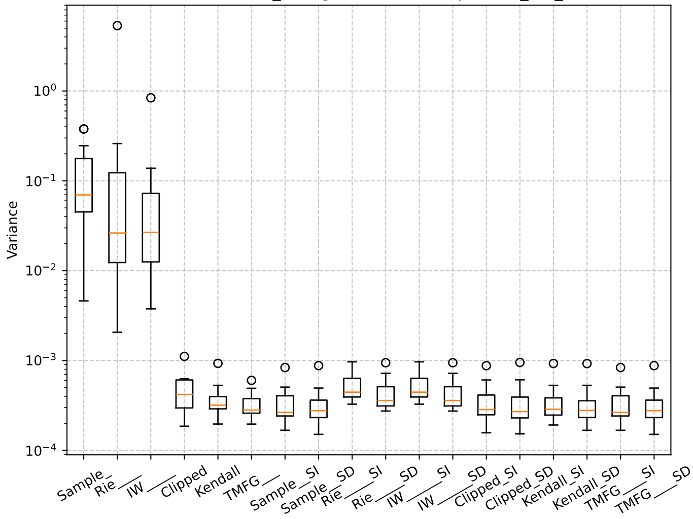
Q=4.00, len_rolling=100: Box Plot per min_var_
