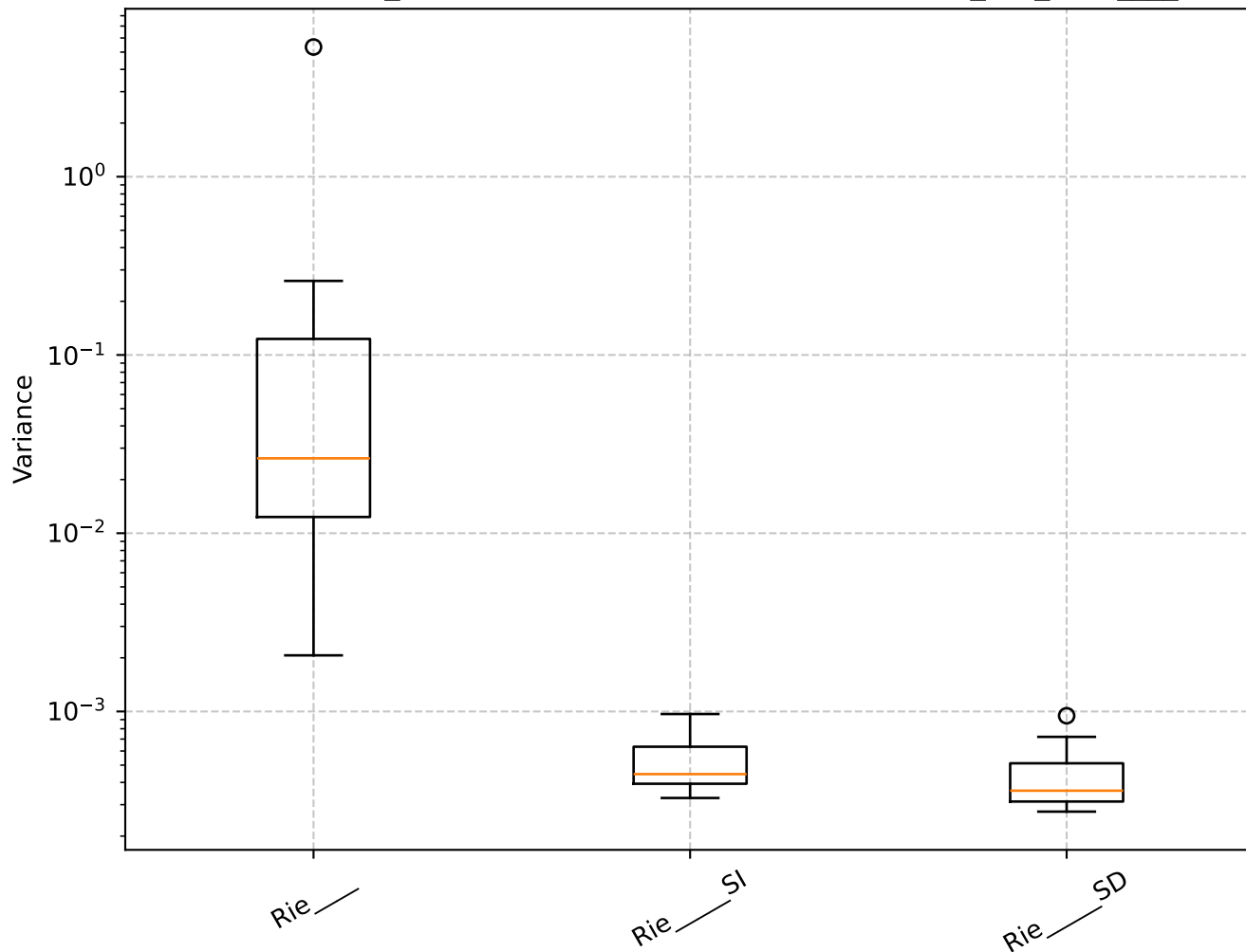
Q=4.00, len_rolling=100: Shrinkage Box Plot - min_var_, Rie____
