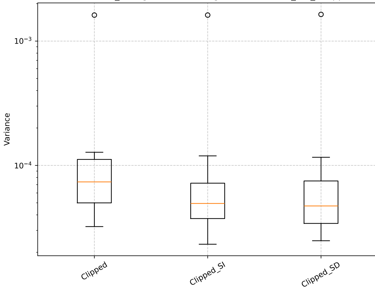
Q=0.50, len_rolling=100: Shrinkage Box Plot - min_var_, Clipped
