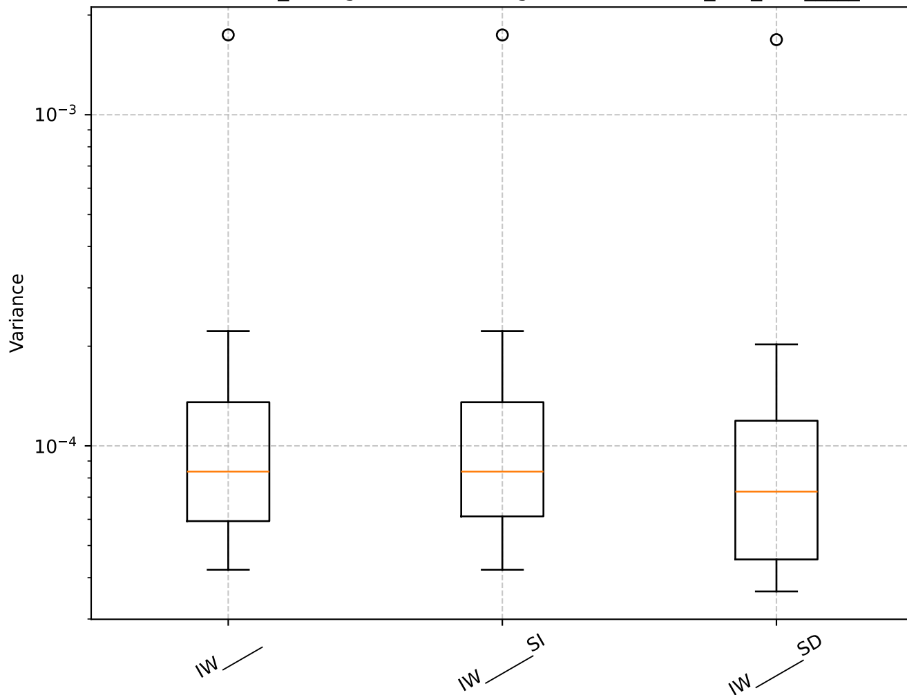
Q=0.50, len_rolling=100: Shrinkage Box Plot - min_var_, IW_____
