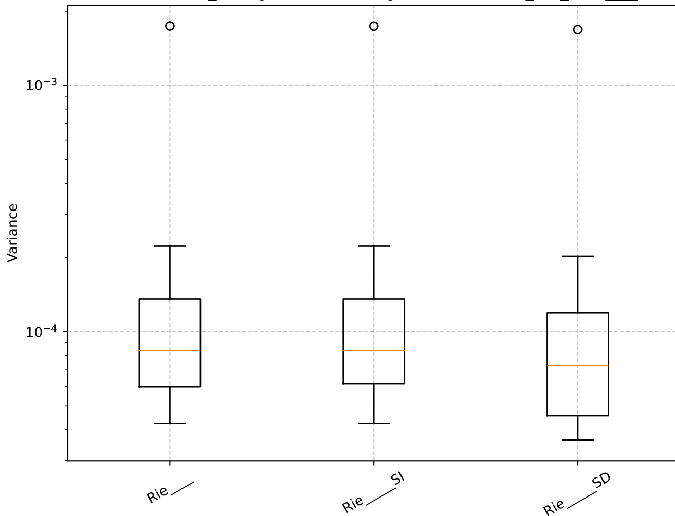
Q=0.51, len_rolling=100: Shrinkage Box Plot - min_var_, Rie____
