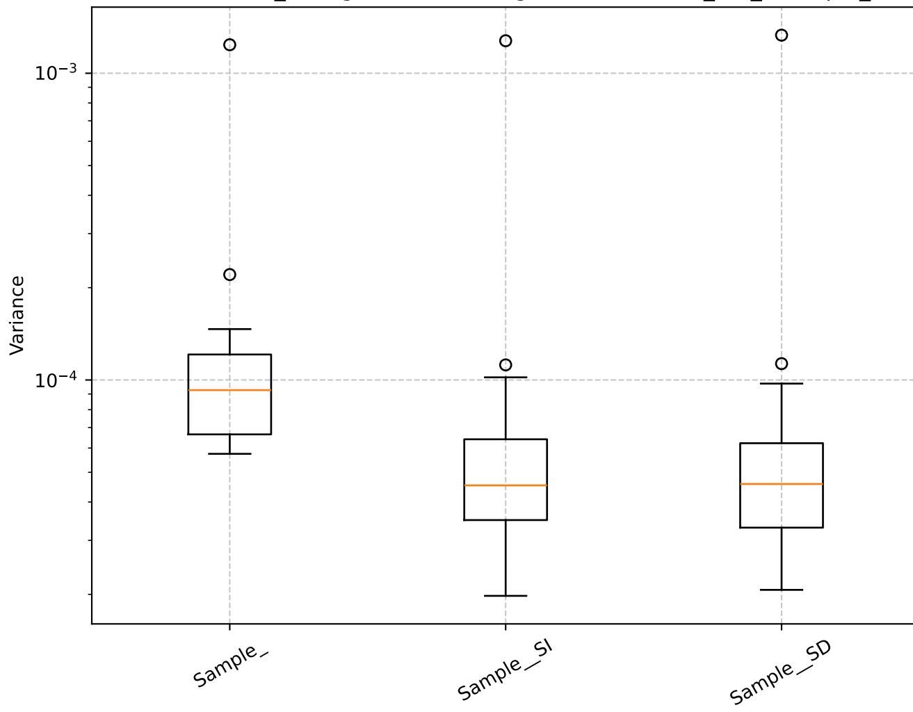
Q=0.51, len_rolling=100: Shrinkage Box Plot - min_var_, Sample_
